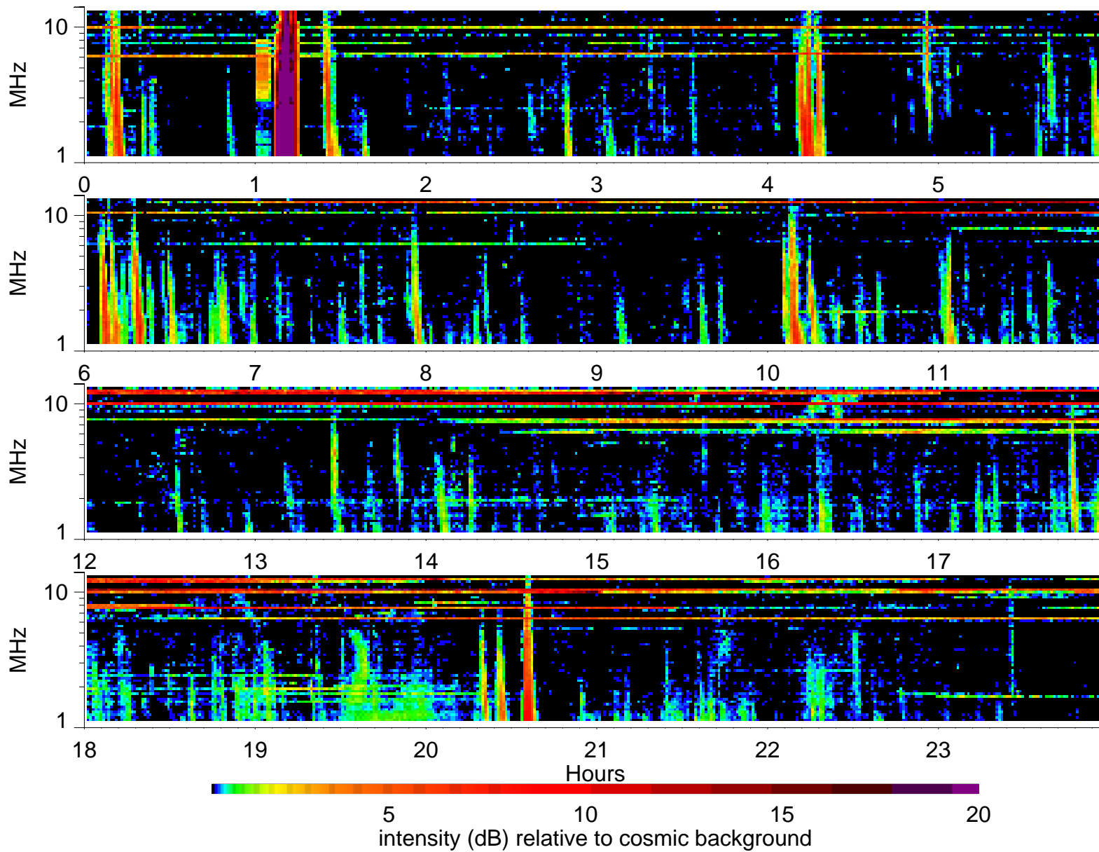
Wind Waves RAD2 receiver: 2004/3/14
