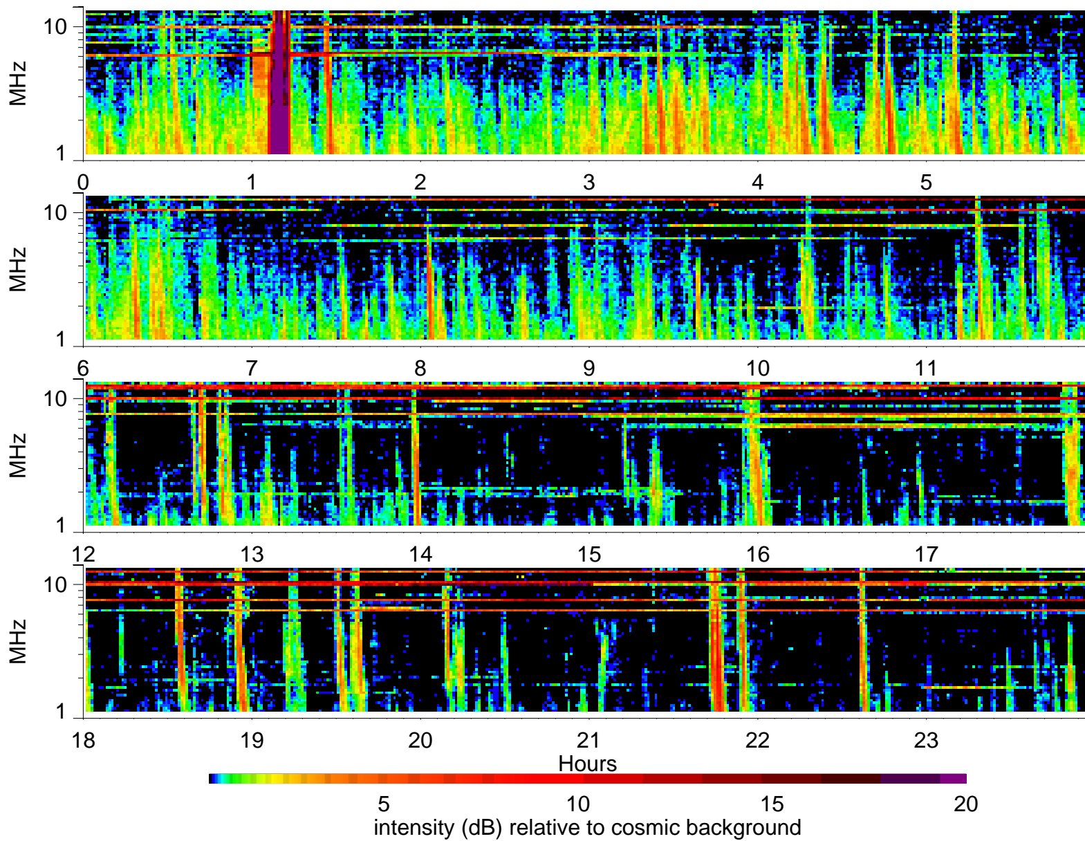
Wind Waves RAD2 receiver: 2004/3/12
