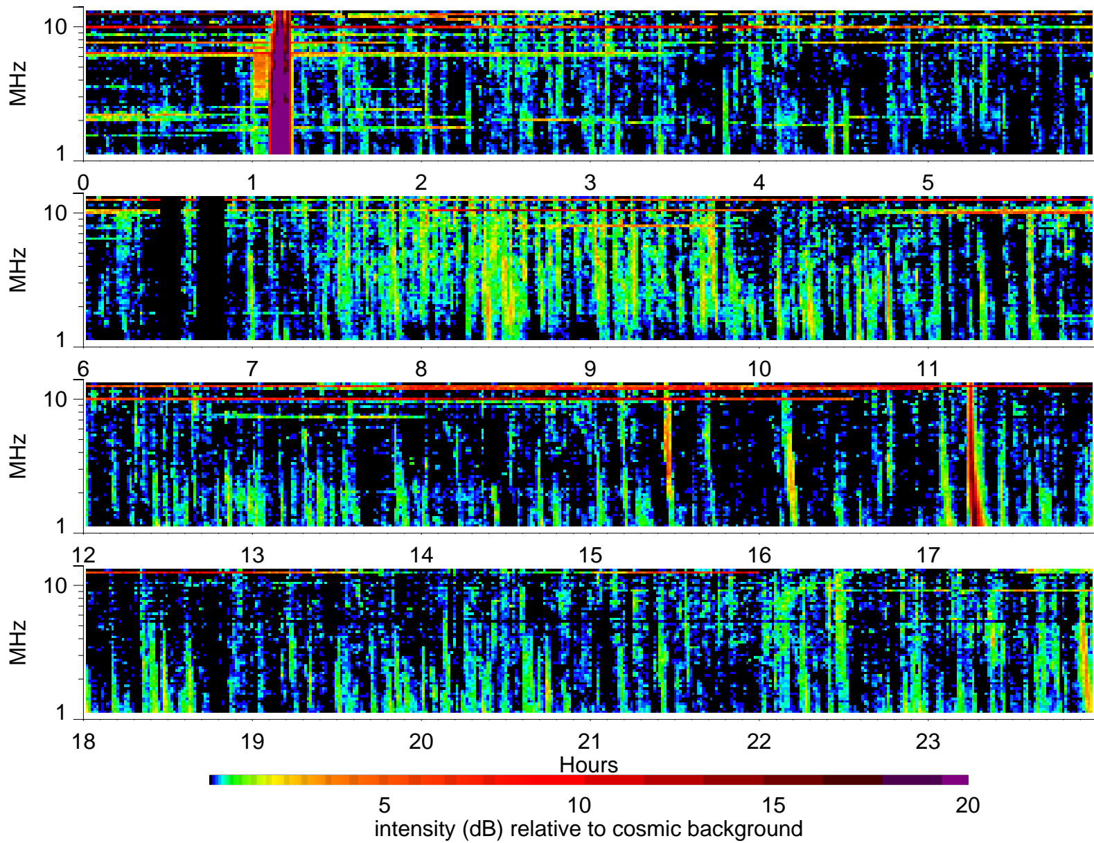
Wind Waves RAD2 receiver: 2004/3/4
