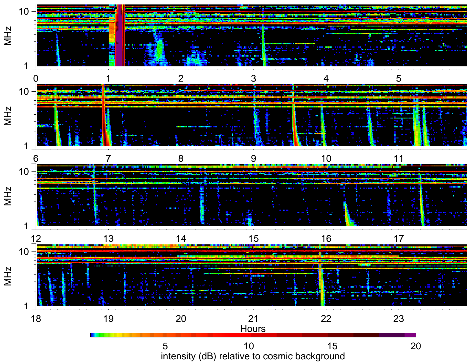
Wind Waves RAD2 receiver: 2004/2/27
