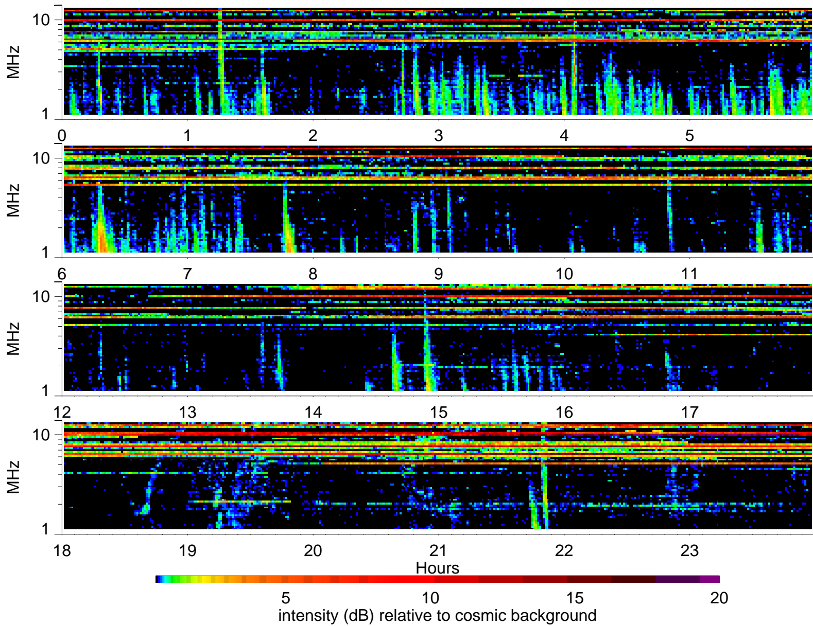
Wind Waves RAD2 receiver: 2004/2/26
