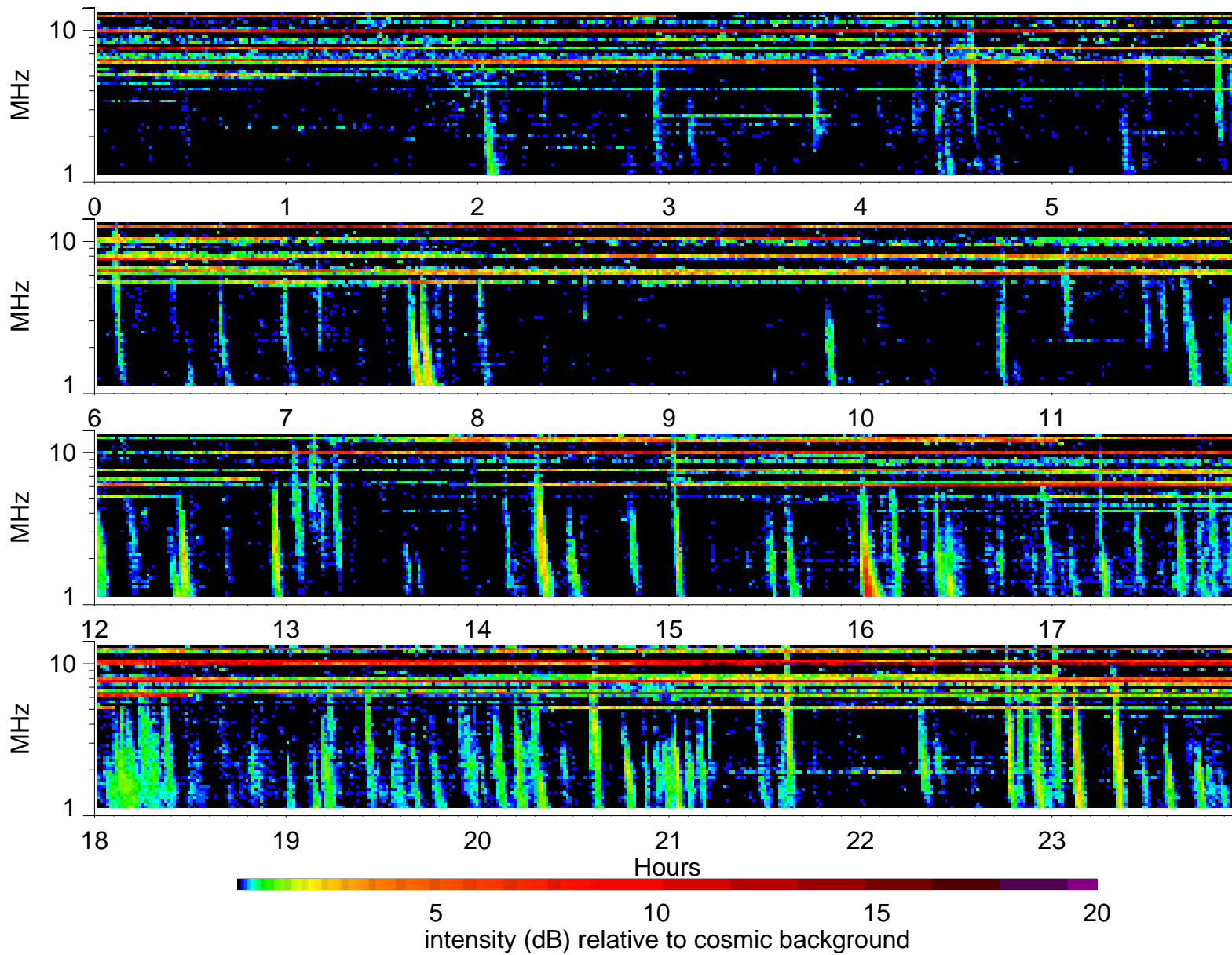
Wind Waves RAD2 receiver: 2004/2/24
