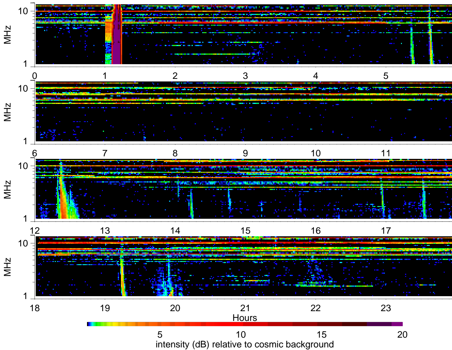
Wind Waves RAD2 receiver: 2004/2/17
