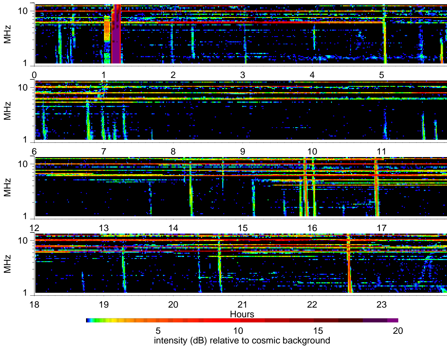
Wind Waves RAD2 receiver: 2004/2/15
