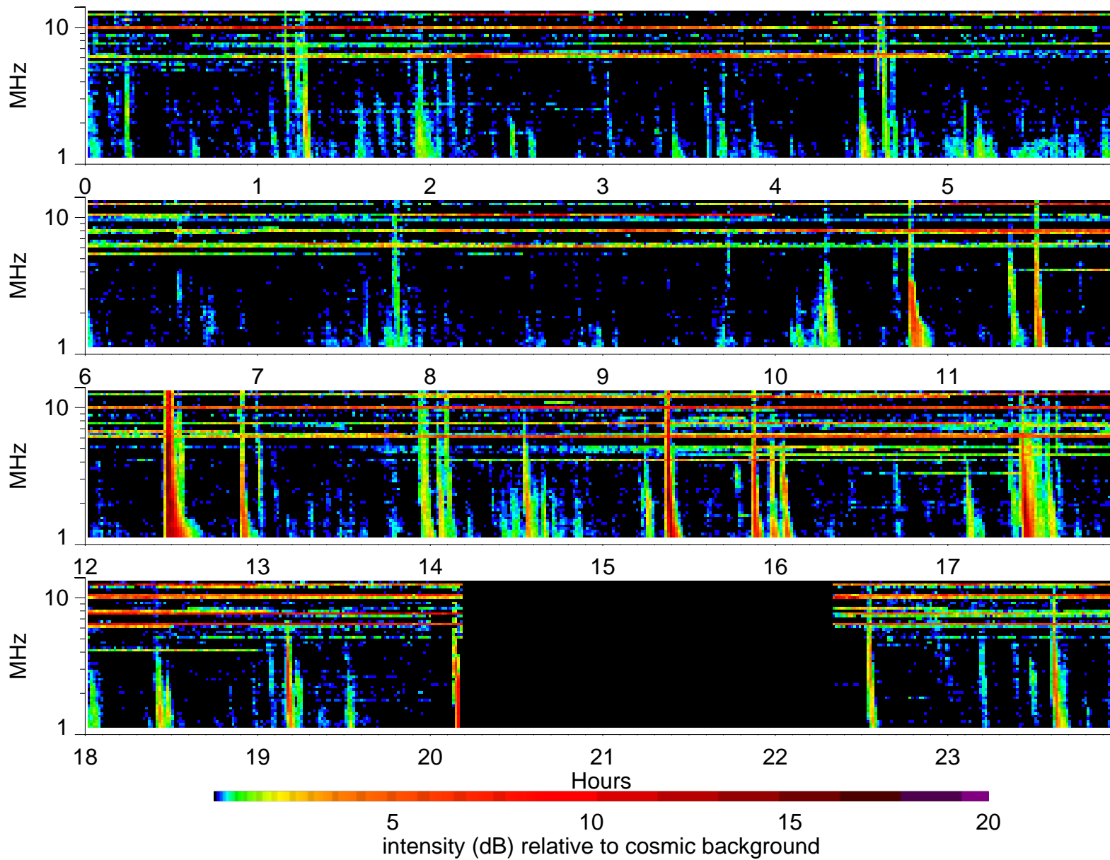
Wind Waves RAD2 receiver: 2004/2/10
