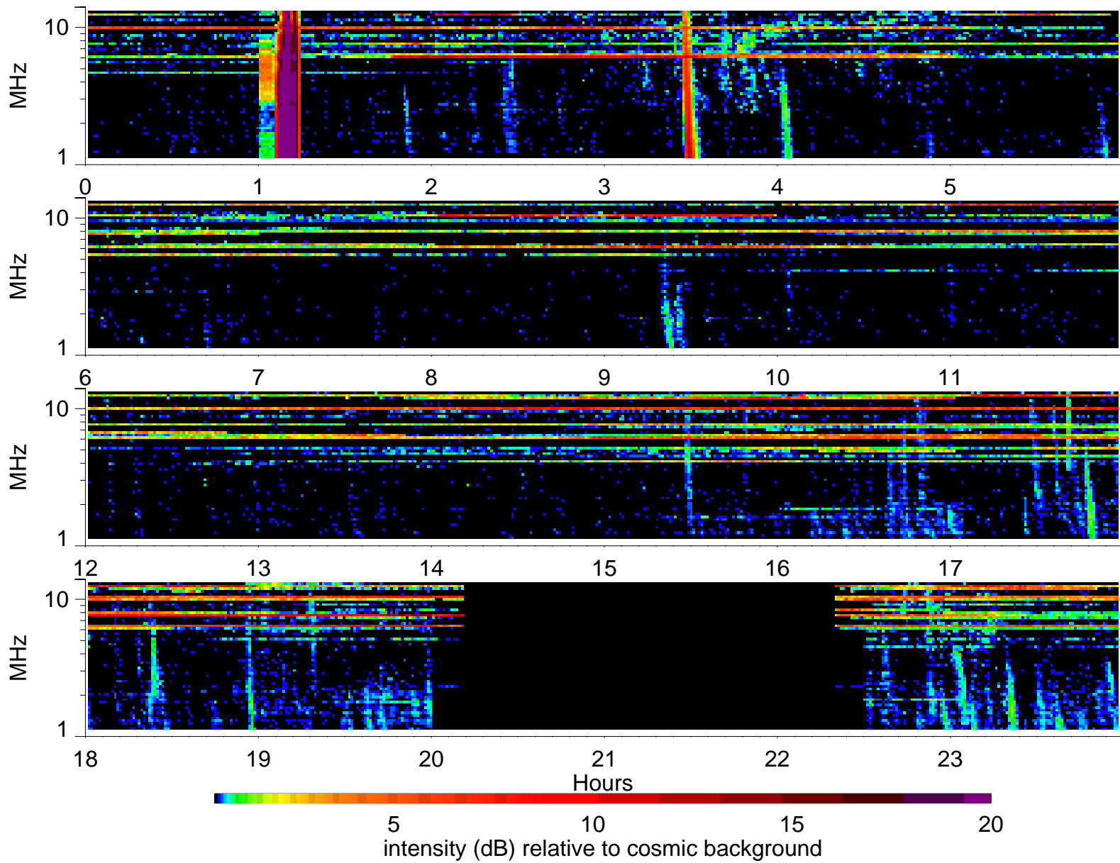
Wind Waves RAD2 receiver: 2004/2/9
