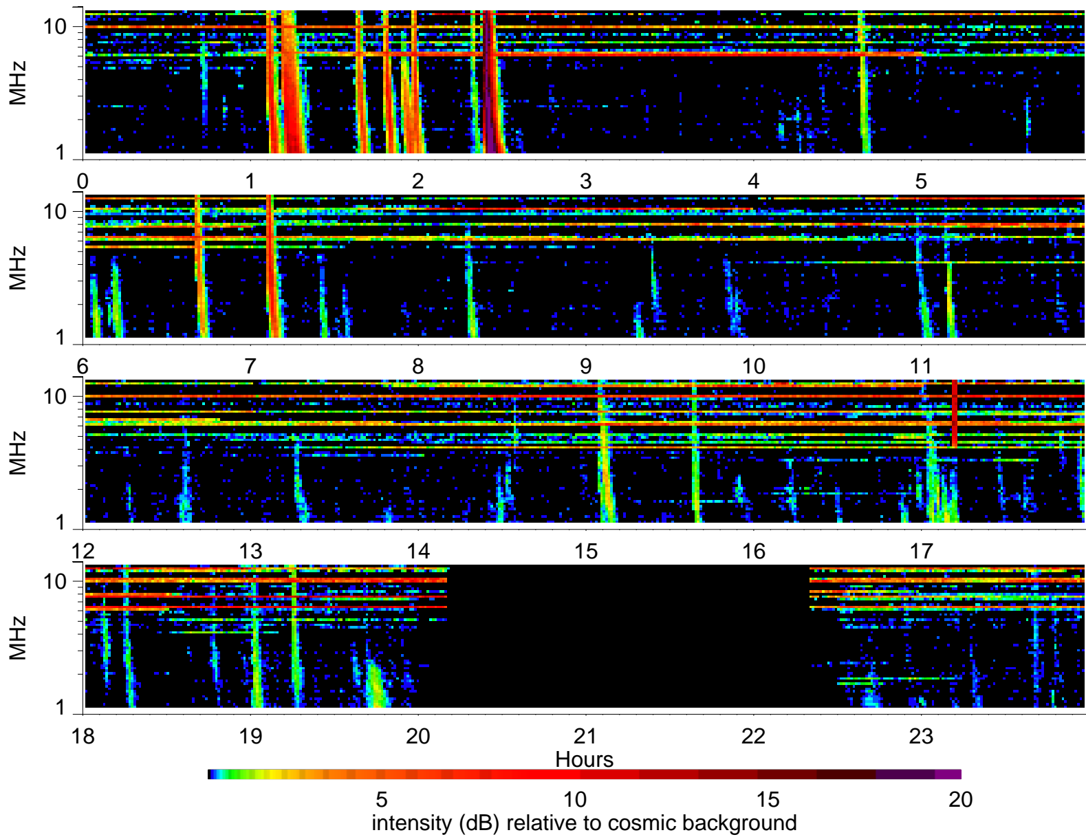
Wind Waves RAD2 receiver: 2004/2/8
