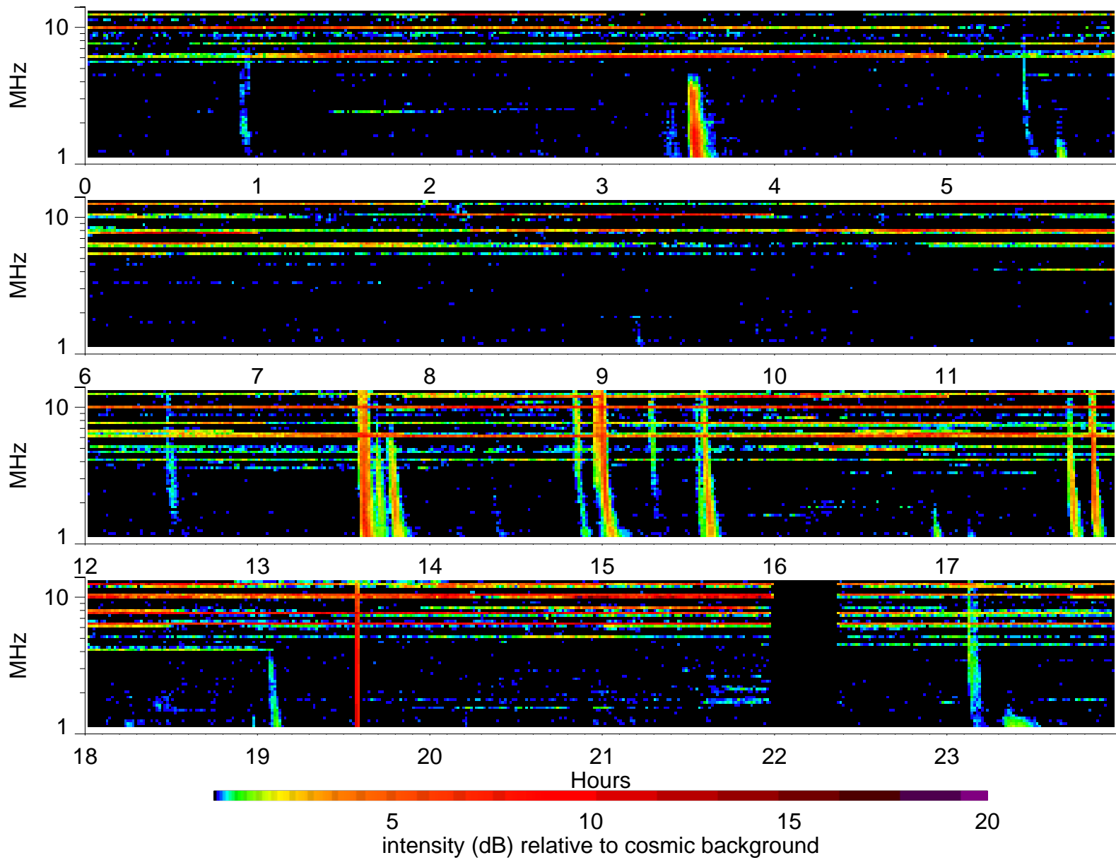
Wind Waves RAD2 receiver: 2004/2/6
