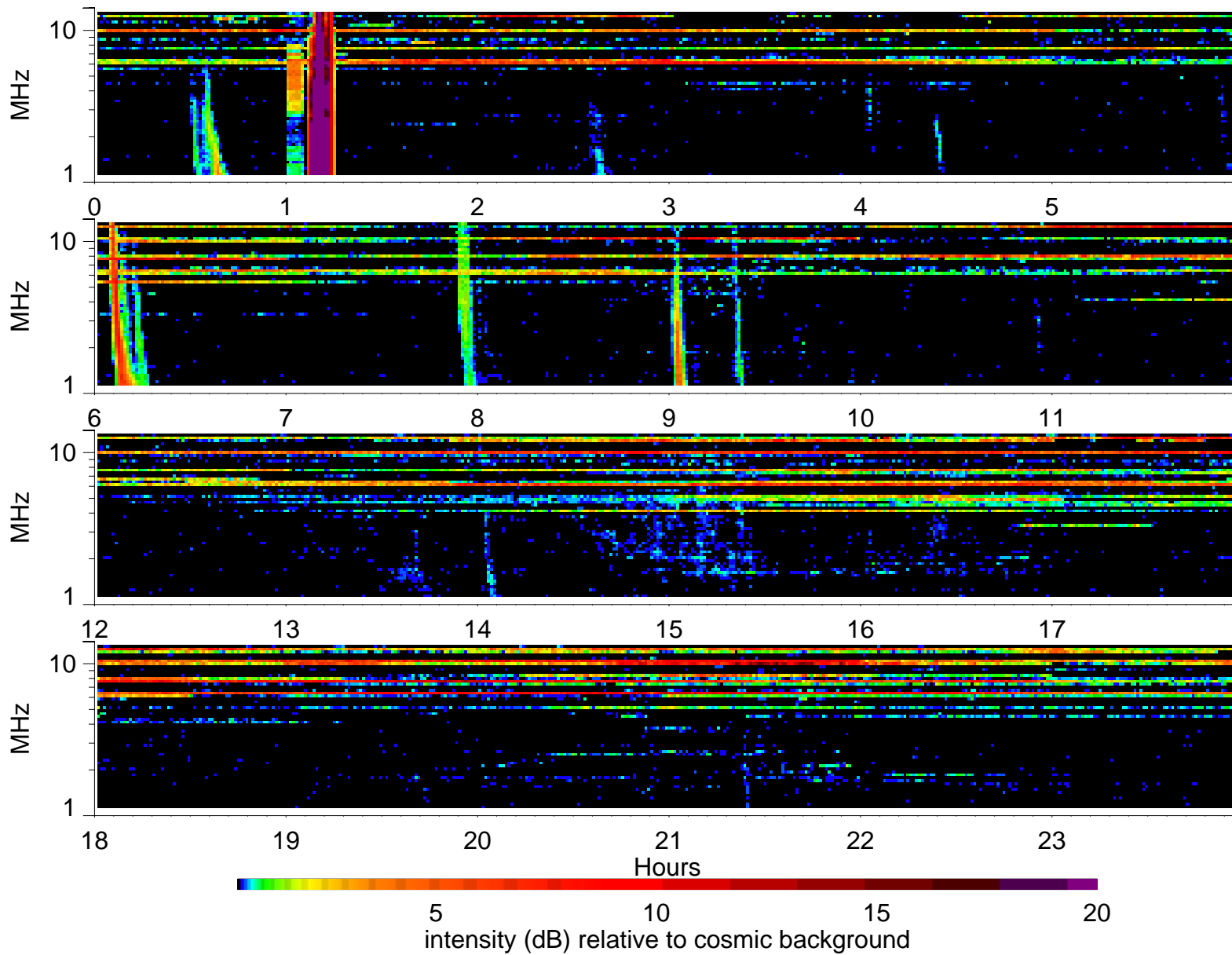
Wind Waves RAD2 receiver: 2004/2/5
