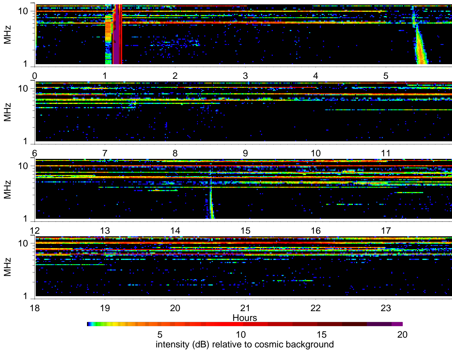
Wind Waves RAD2 receiver: 2004/1/30
