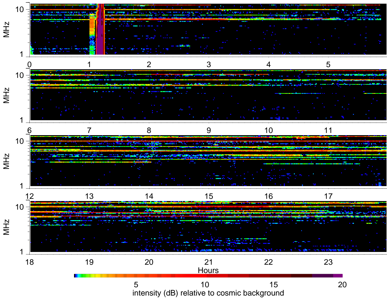
Wind Waves RAD2 receiver: 2004/1/28
