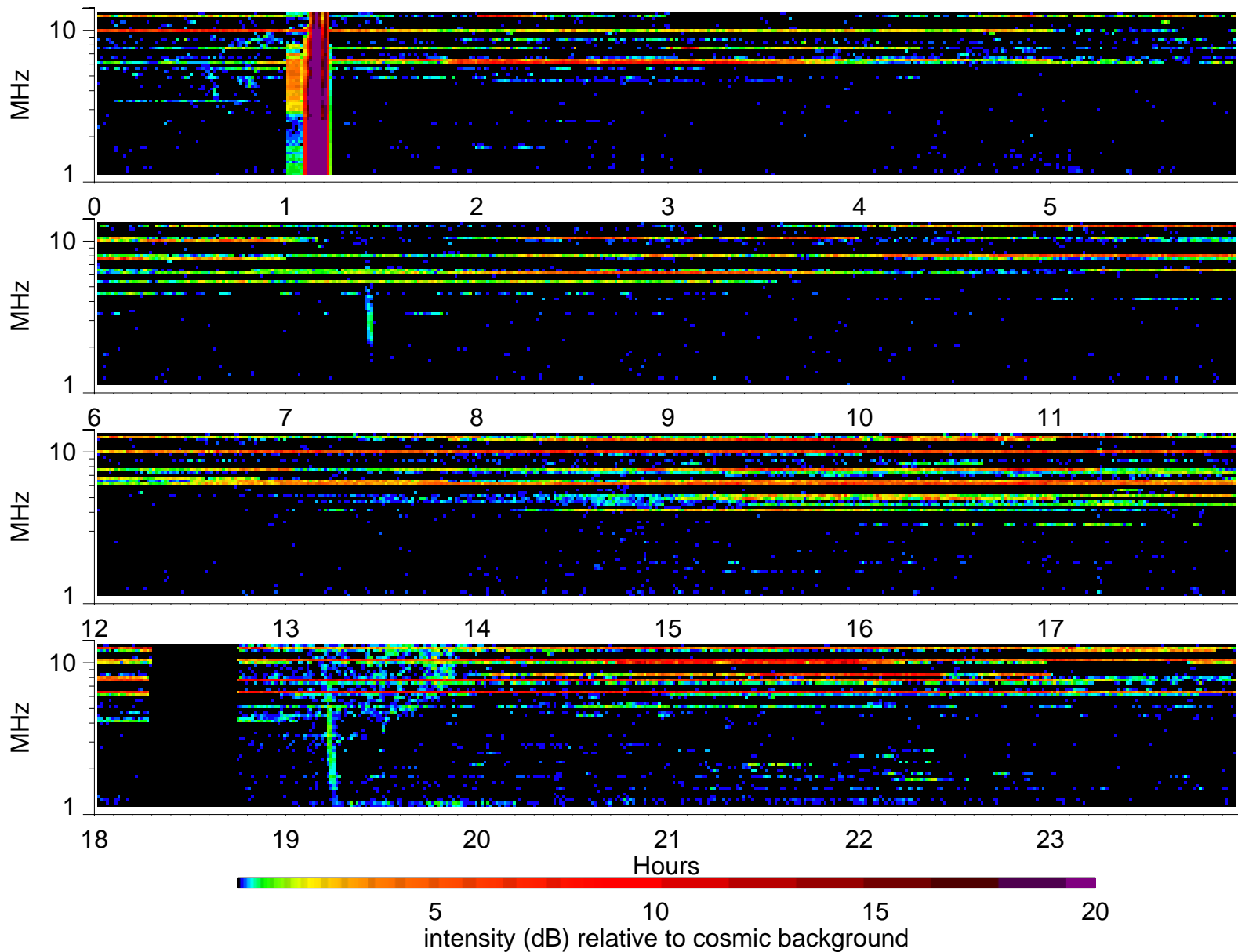
Wind Waves RAD2 receiver: 2004/1/26
