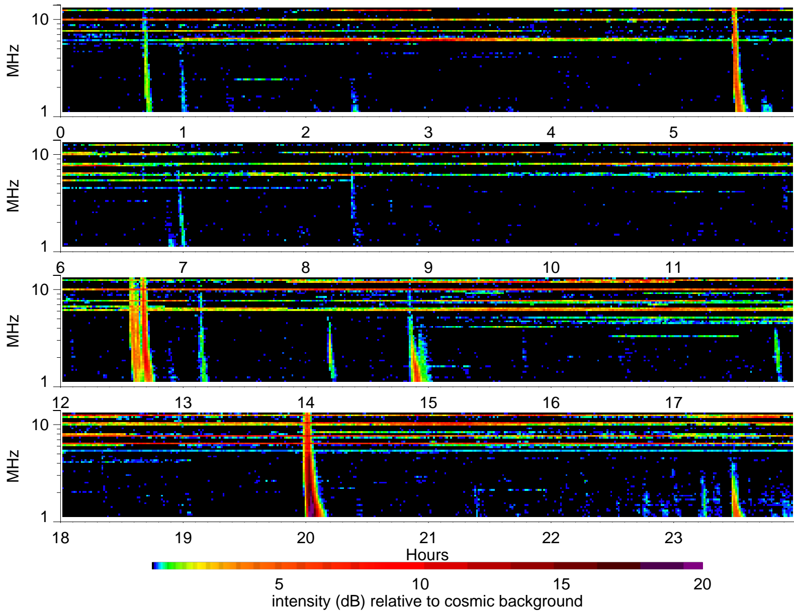
Wind Waves RAD2 receiver: 2004/1/19
