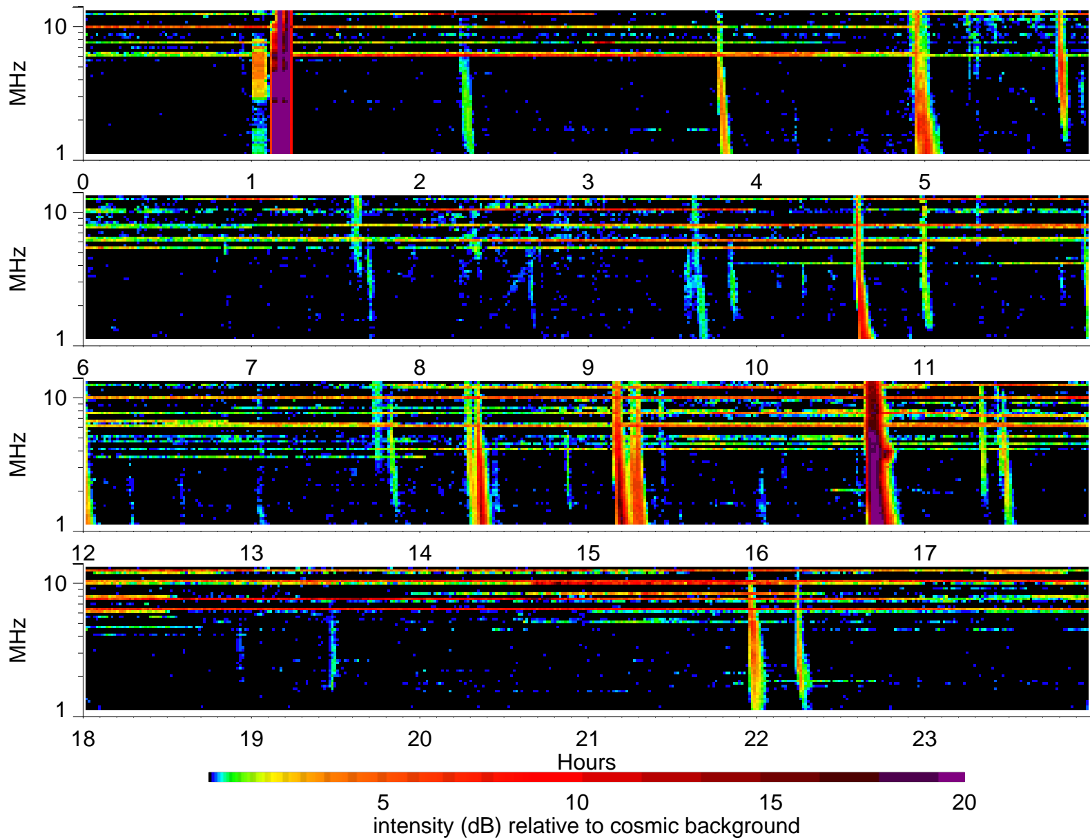
Wind Waves RAD2 receiver: 2004/1/8
