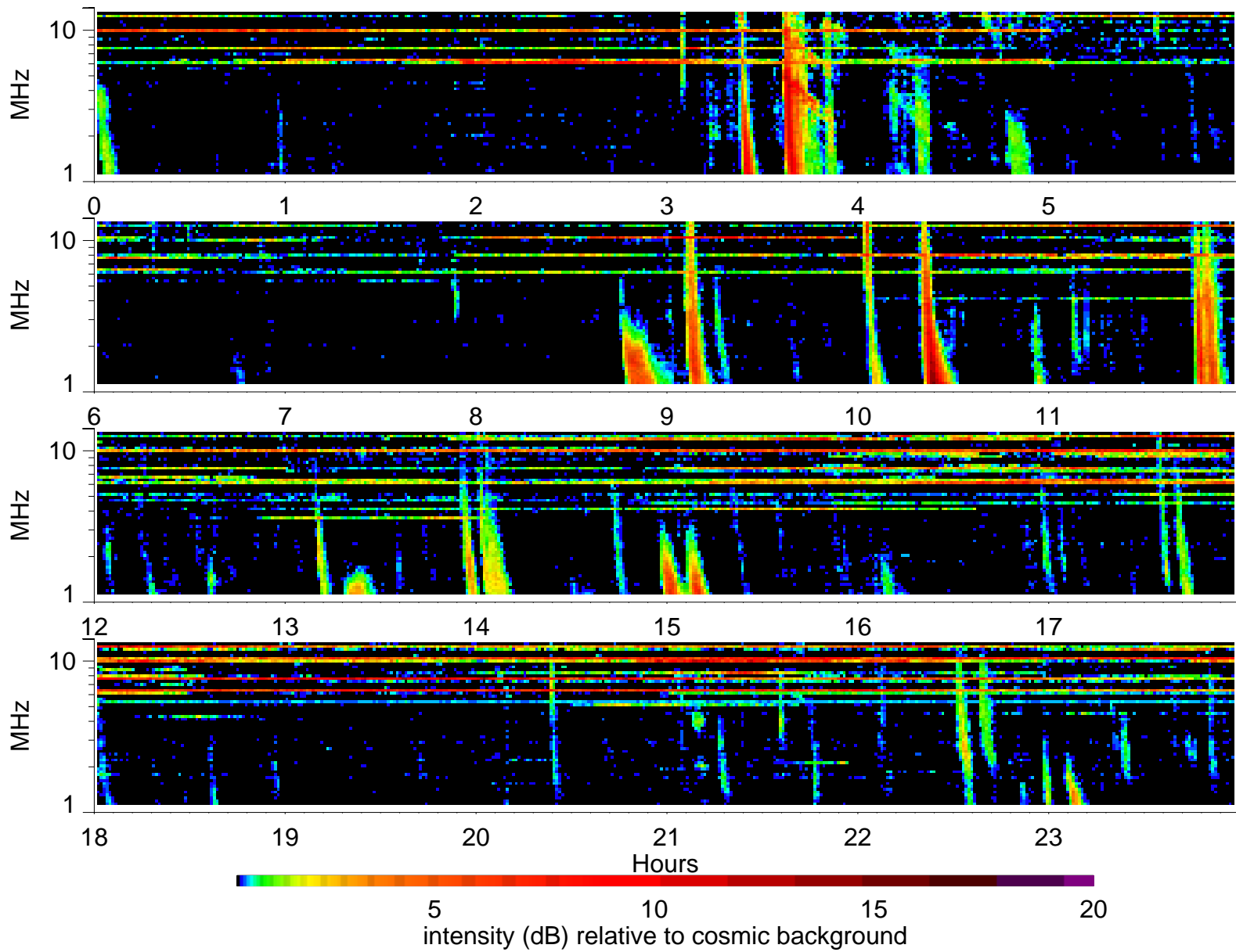
Wind Waves RAD2 receiver: 2004/1/5
