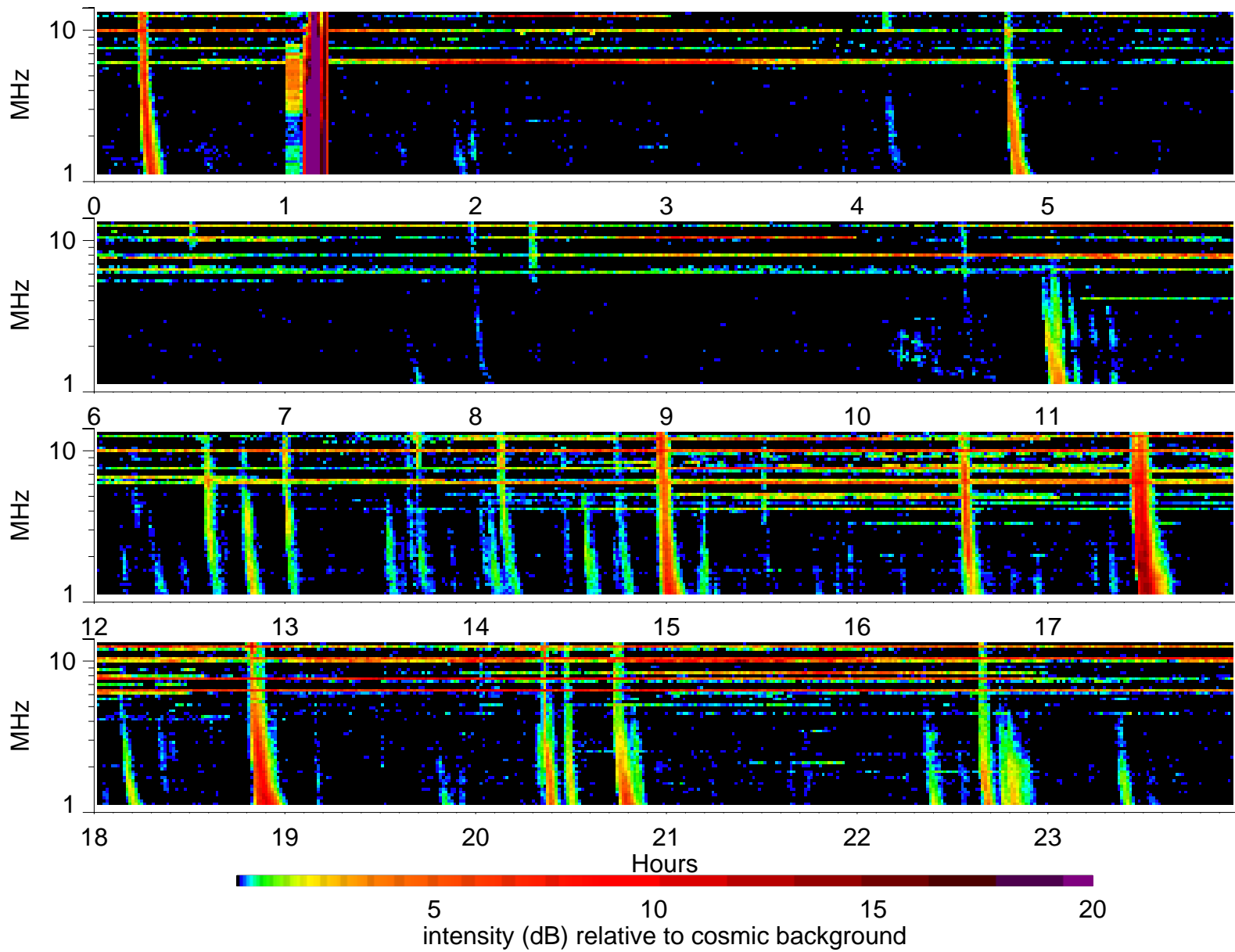
Wind Waves RAD2 receiver: 2004/1/4
