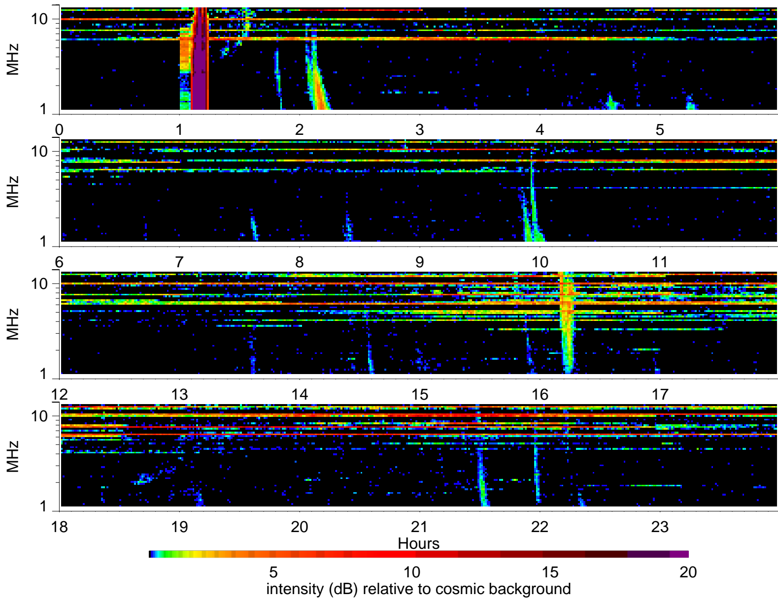
Wind Waves RAD2 receiver: 2004/1/2
