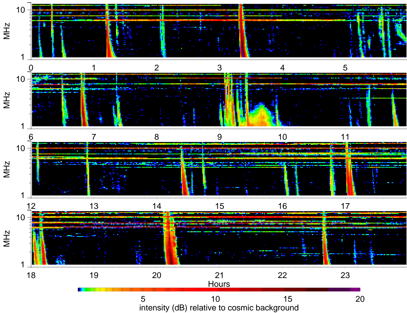
Wind Waves RAD2 receiver: 2004/1/1
