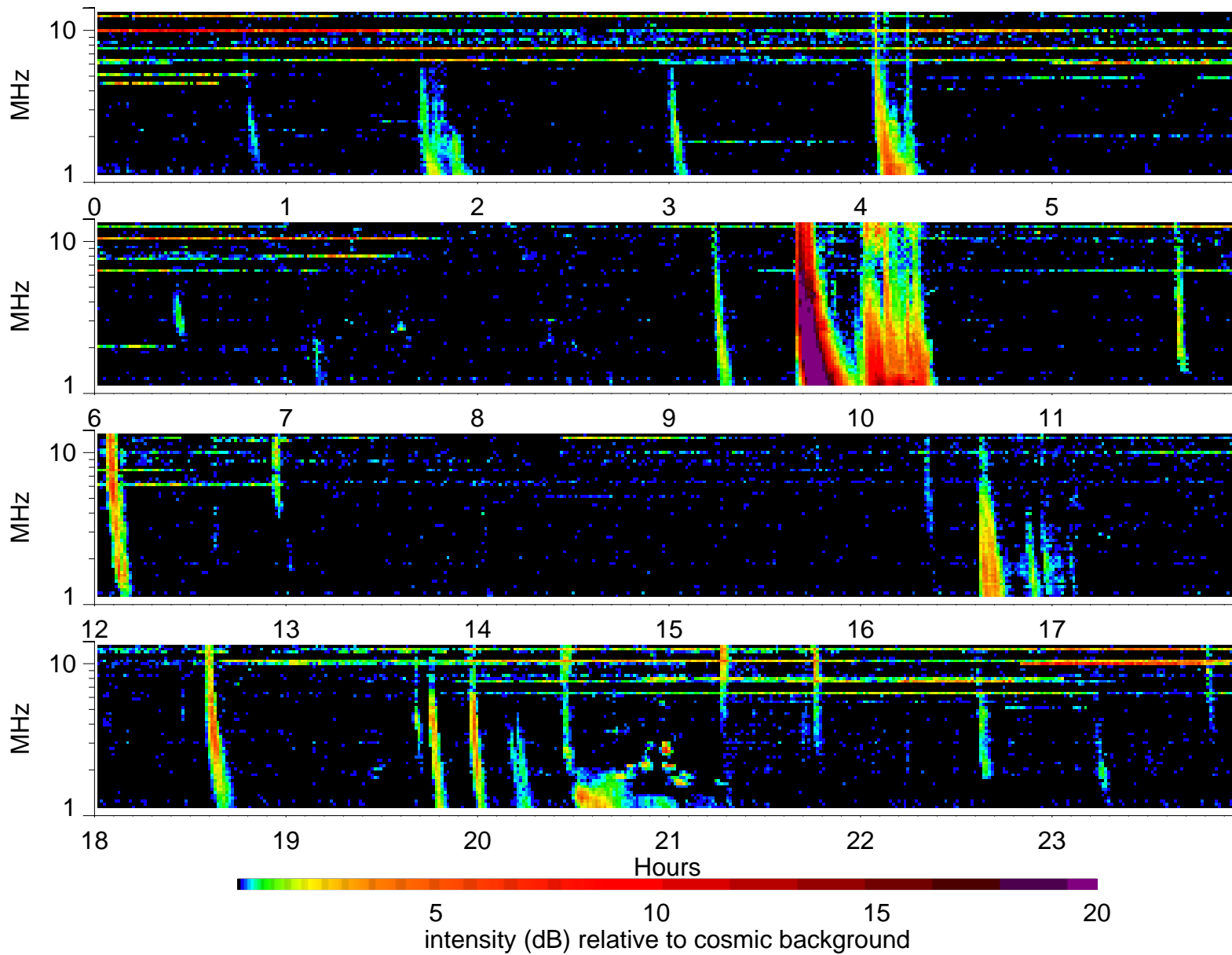
Wind Waves RAD2 receiver: 2001/12/29
