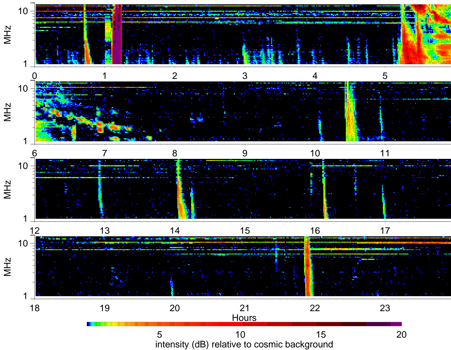
Wind Waves RAD2 receiver: 2001/12/26
