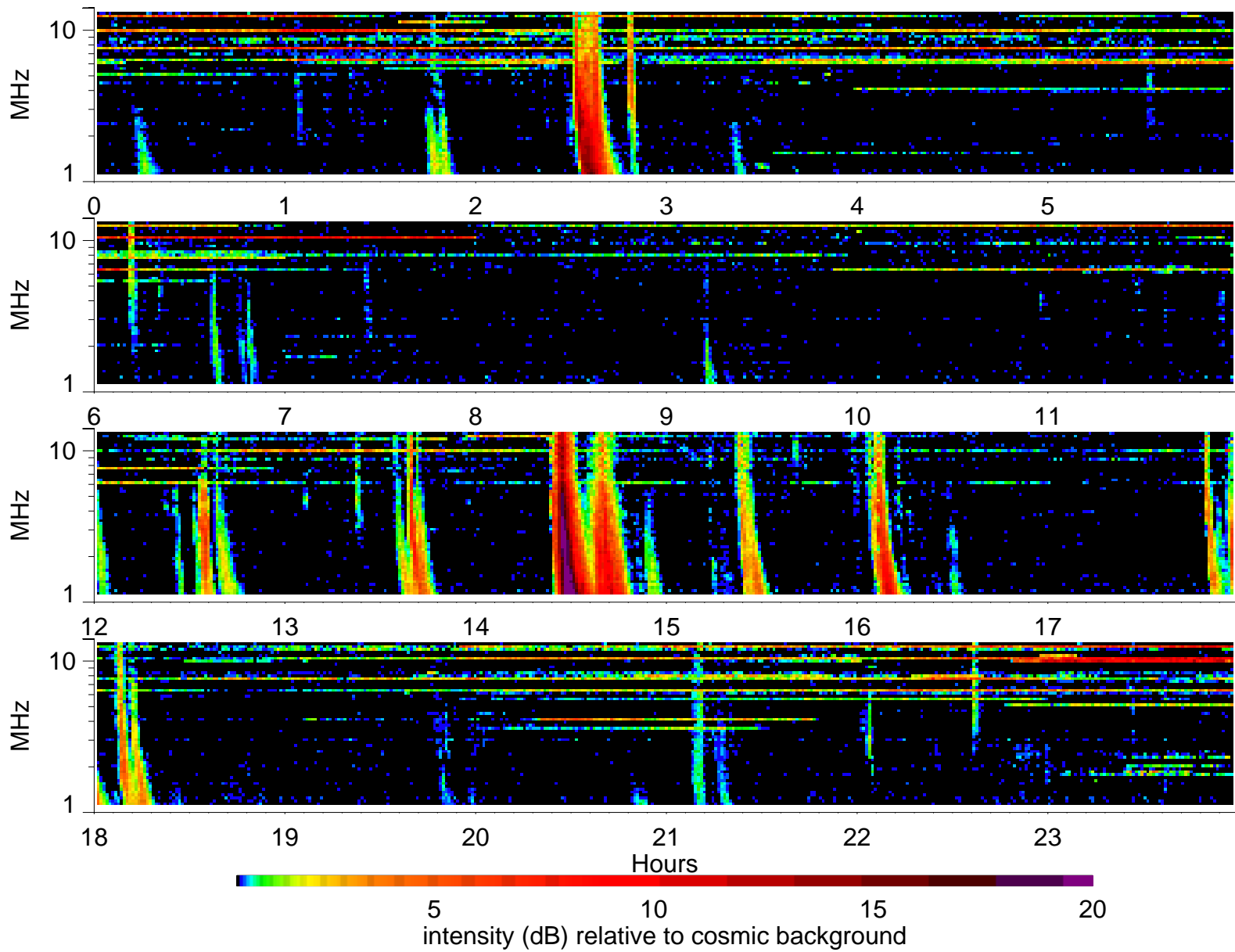
Wind Waves RAD2 receiver: 2001/12/13
