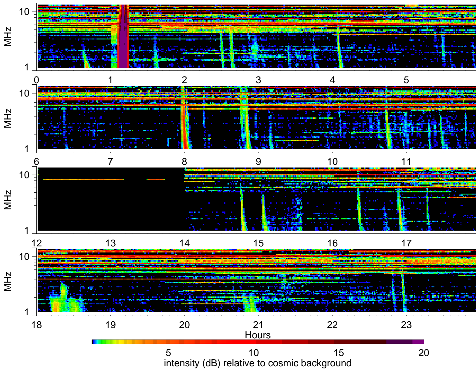
Wind Waves RAD2 receiver: 2001/12/4
