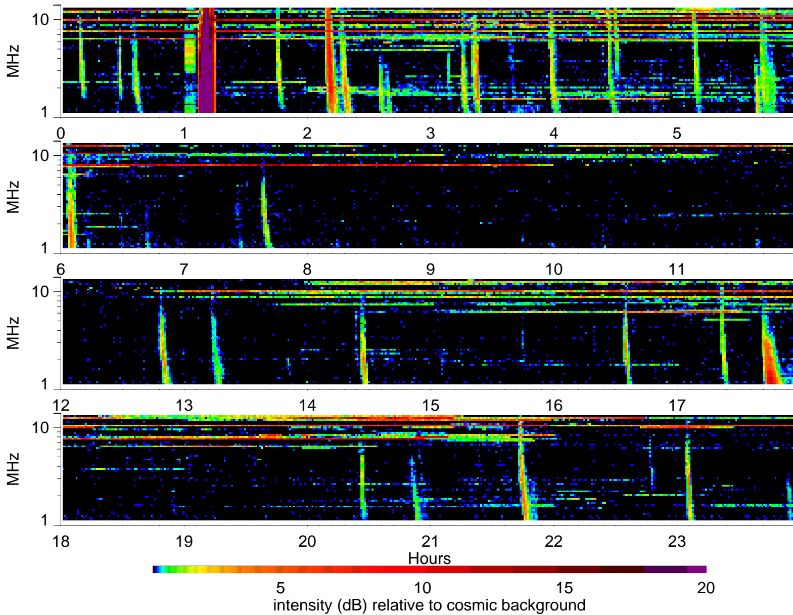
Wind Waves RAD2 receiver: 2001/11/30
