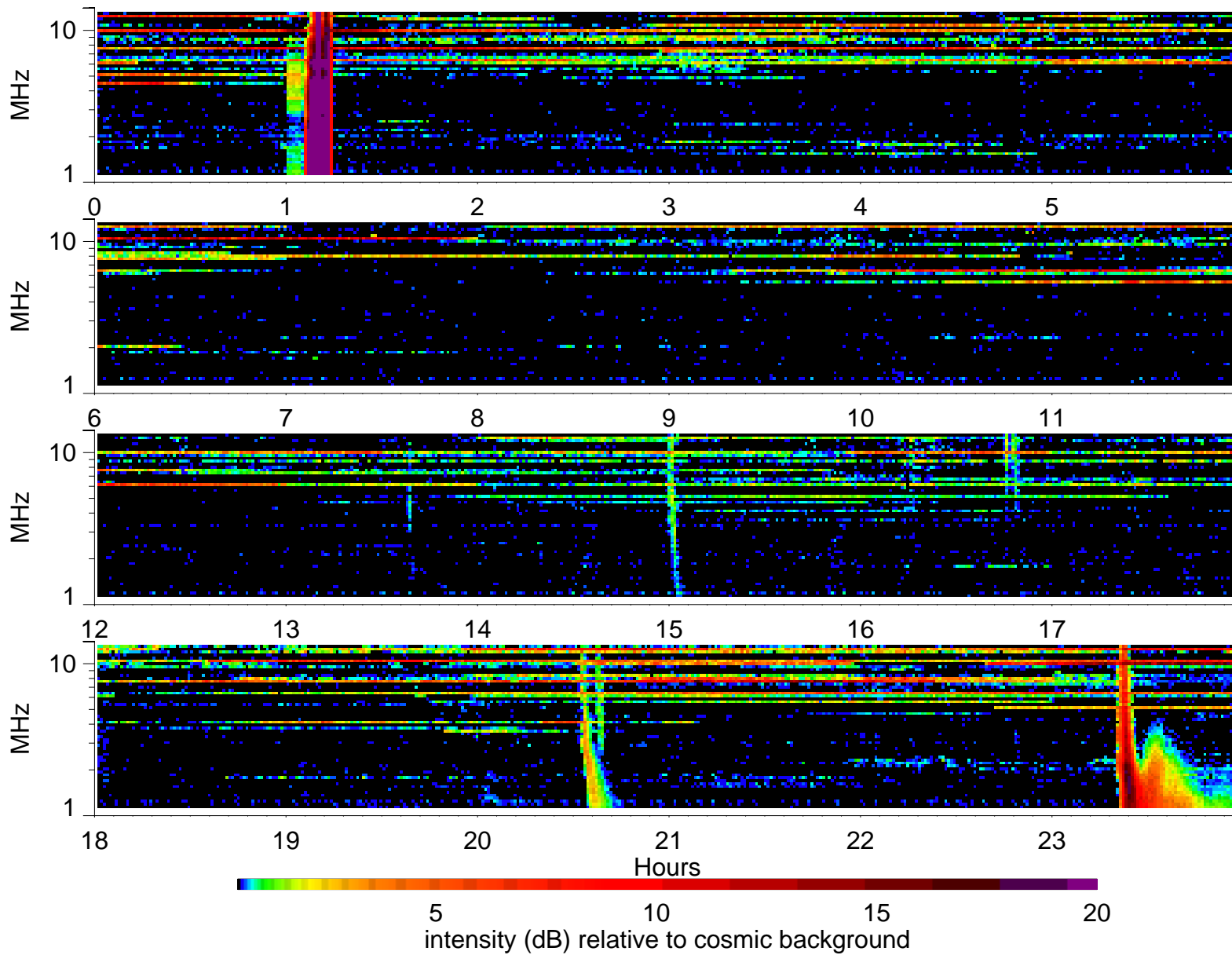
Wind Waves RAD2 receiver: 2001/11/26
