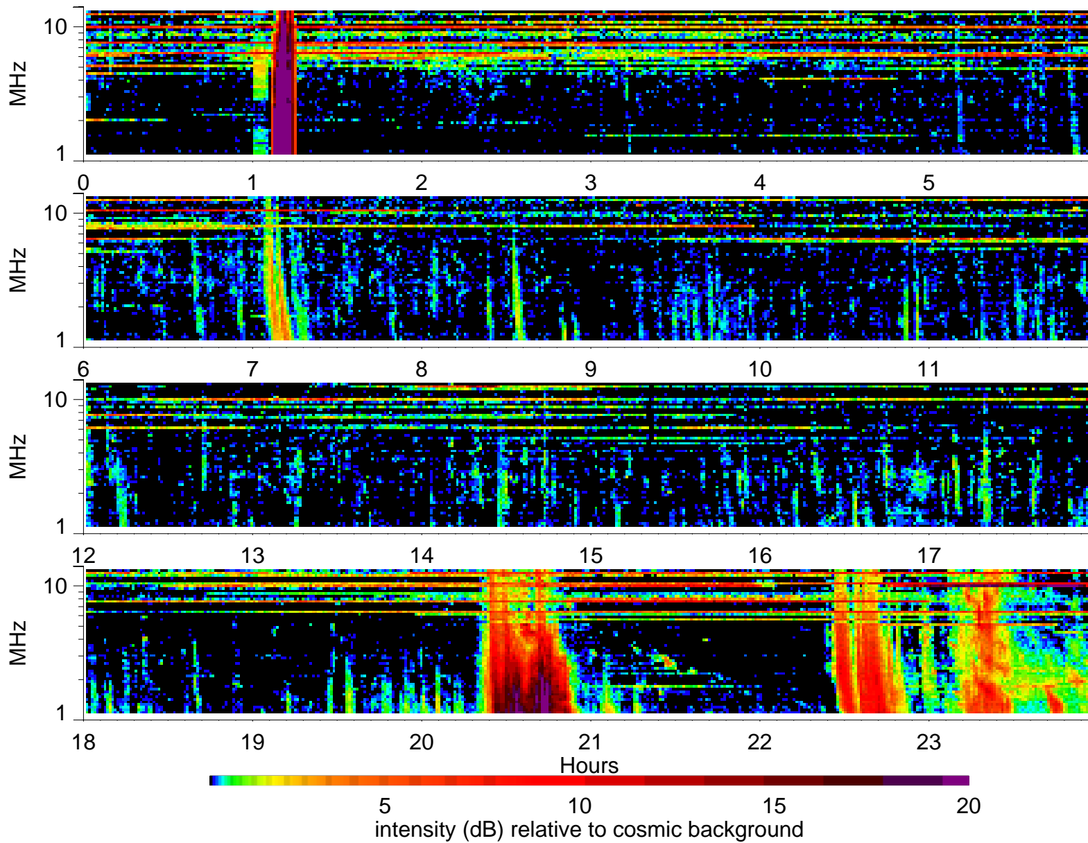
Wind Waves RAD2 receiver: 2001/11/22
