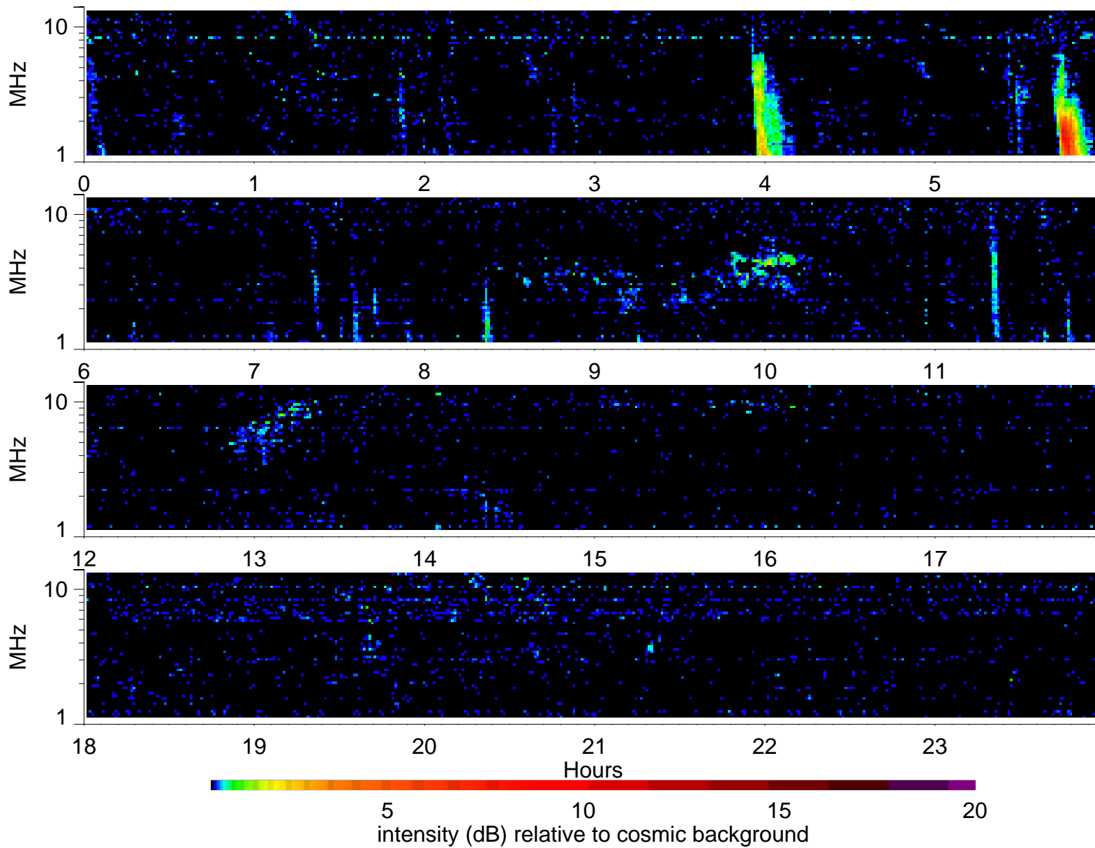
Wind Waves RAD2 receiver: 2001/11/13
