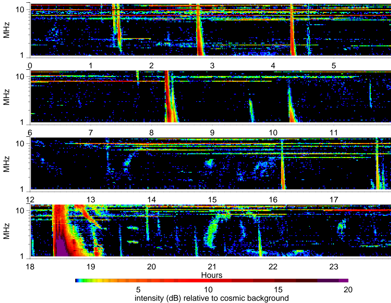
Wind Waves RAD2 receiver: 2001/11/9
