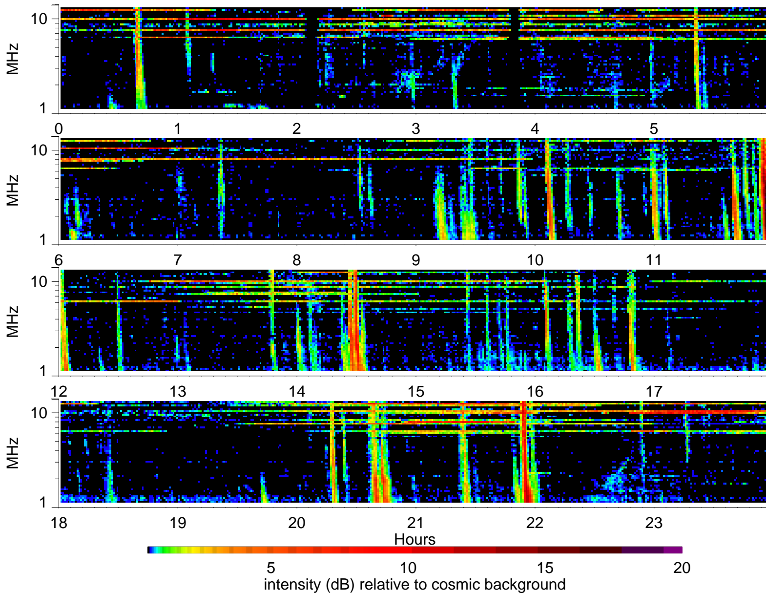
Wind Waves RAD2 receiver: 2001/11/5
