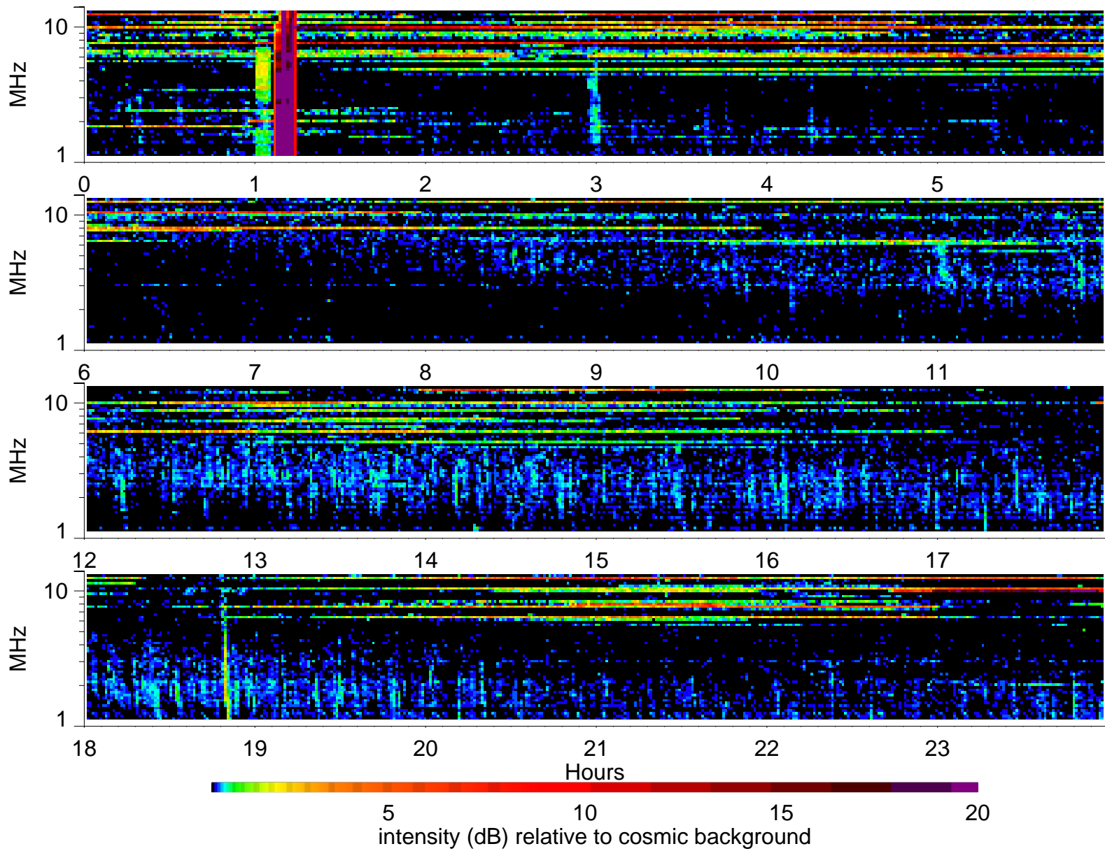
Wind Waves RAD2 receiver: 2001/11/2
