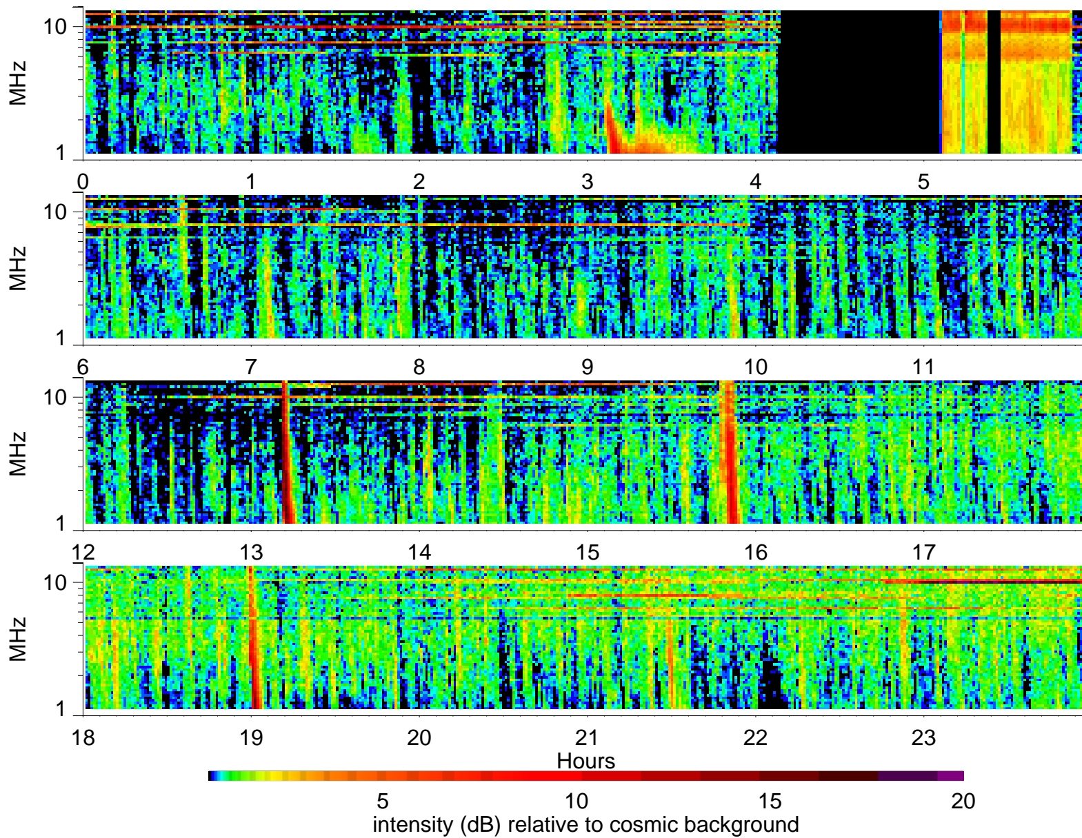
Wind Waves RAD2 receiver: 2001/10/30
