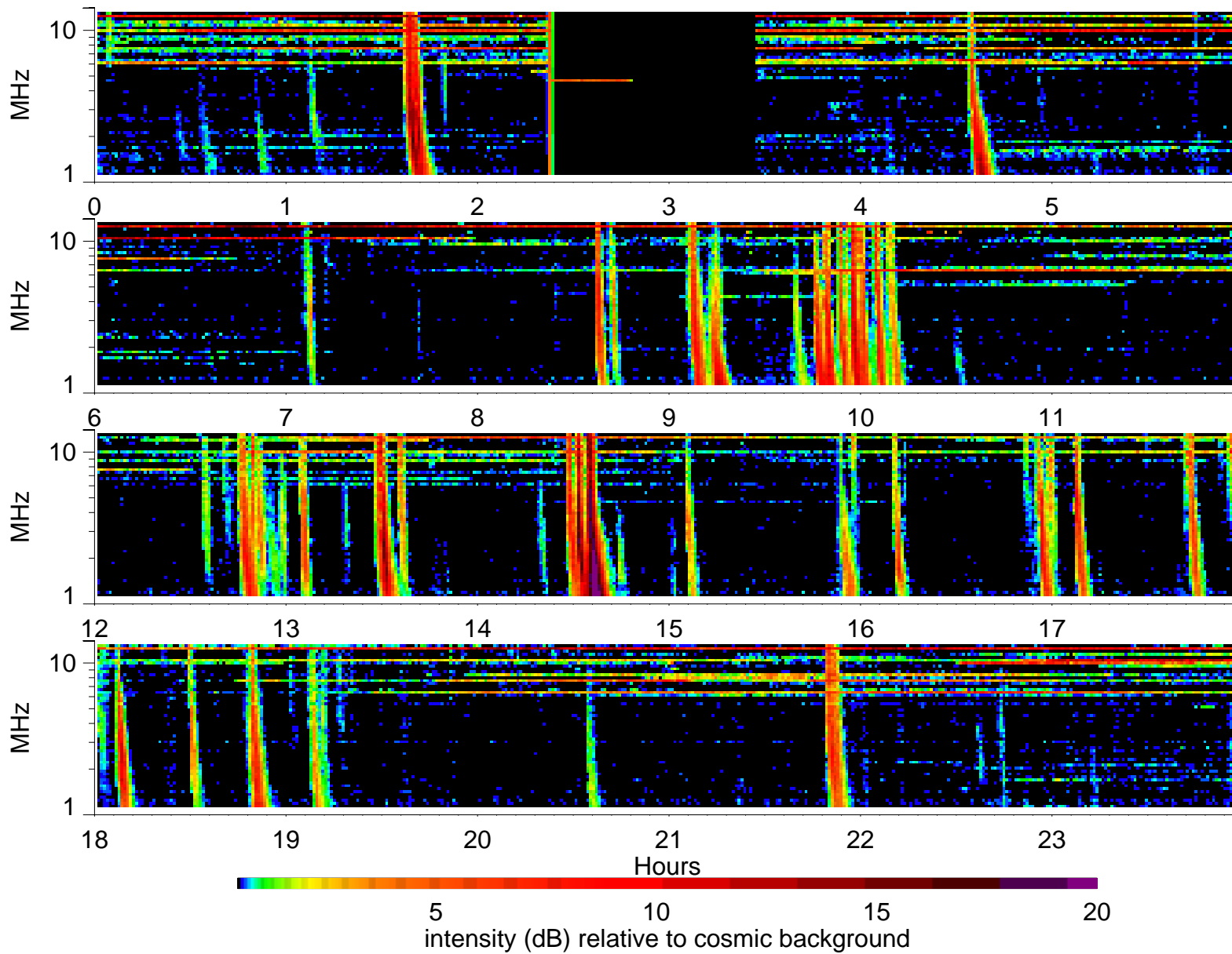
Wind Waves RAD2 receiver: 2001/10/26
