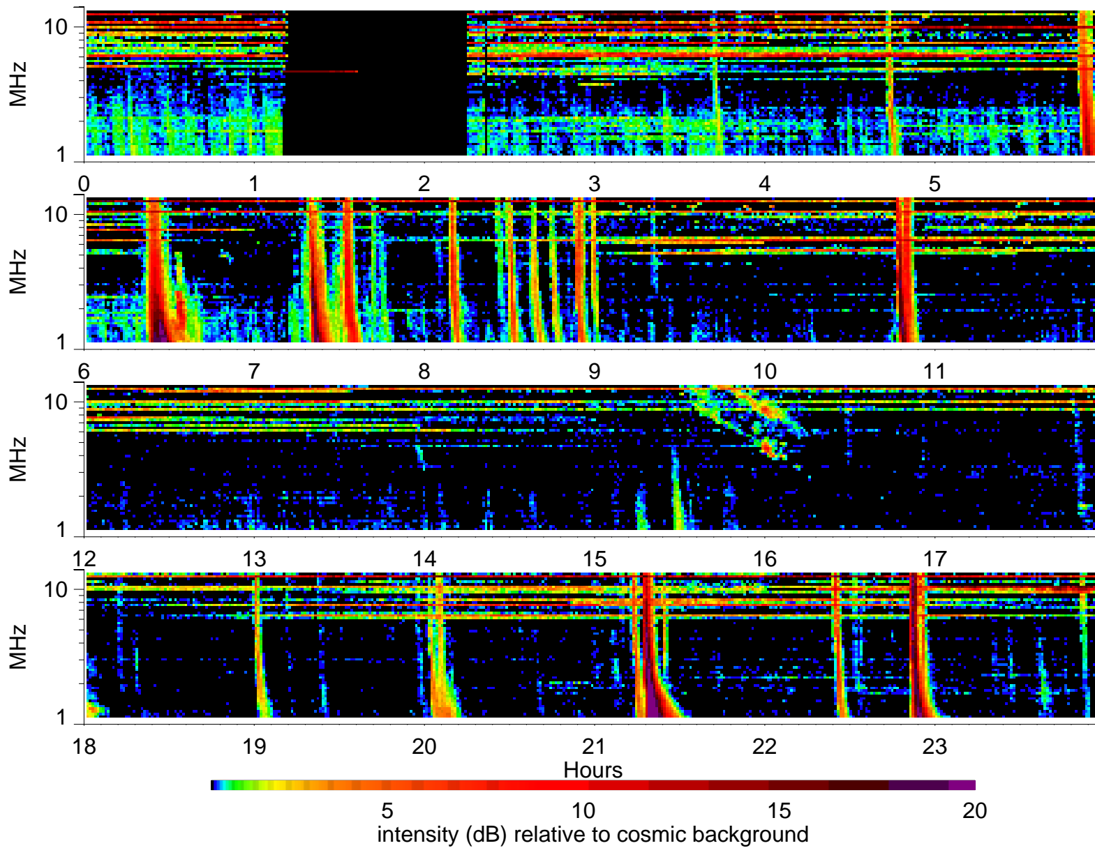
Wind Waves RAD2 receiver: 2001/10/25
