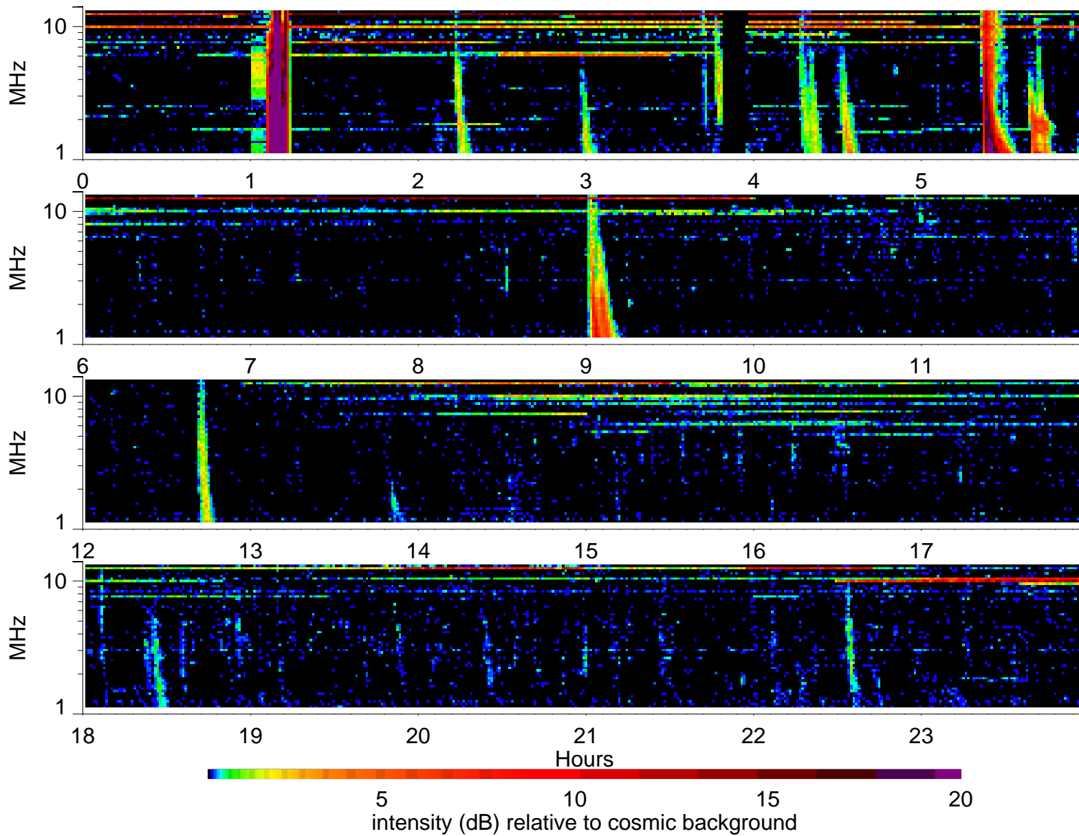
Wind Waves RAD2 receiver: 2001/10/13
