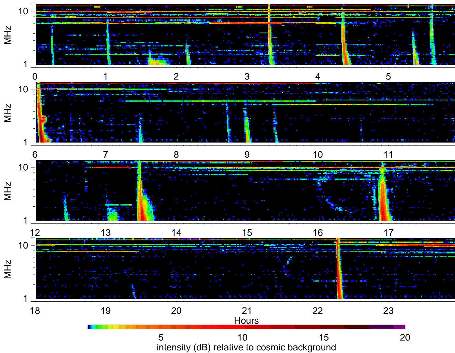
Wind Waves RAD2 receiver: 2001/10/12
