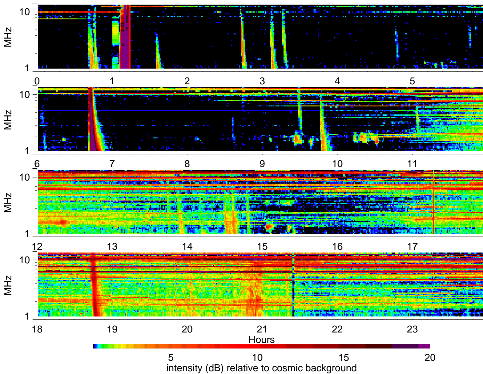
Wind Waves RAD2 receiver: 2001/10/3
