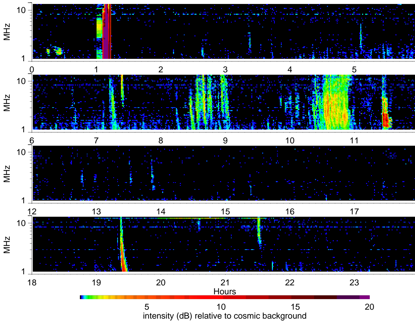
Wind Waves RAD2 receiver: 2001/9/29
