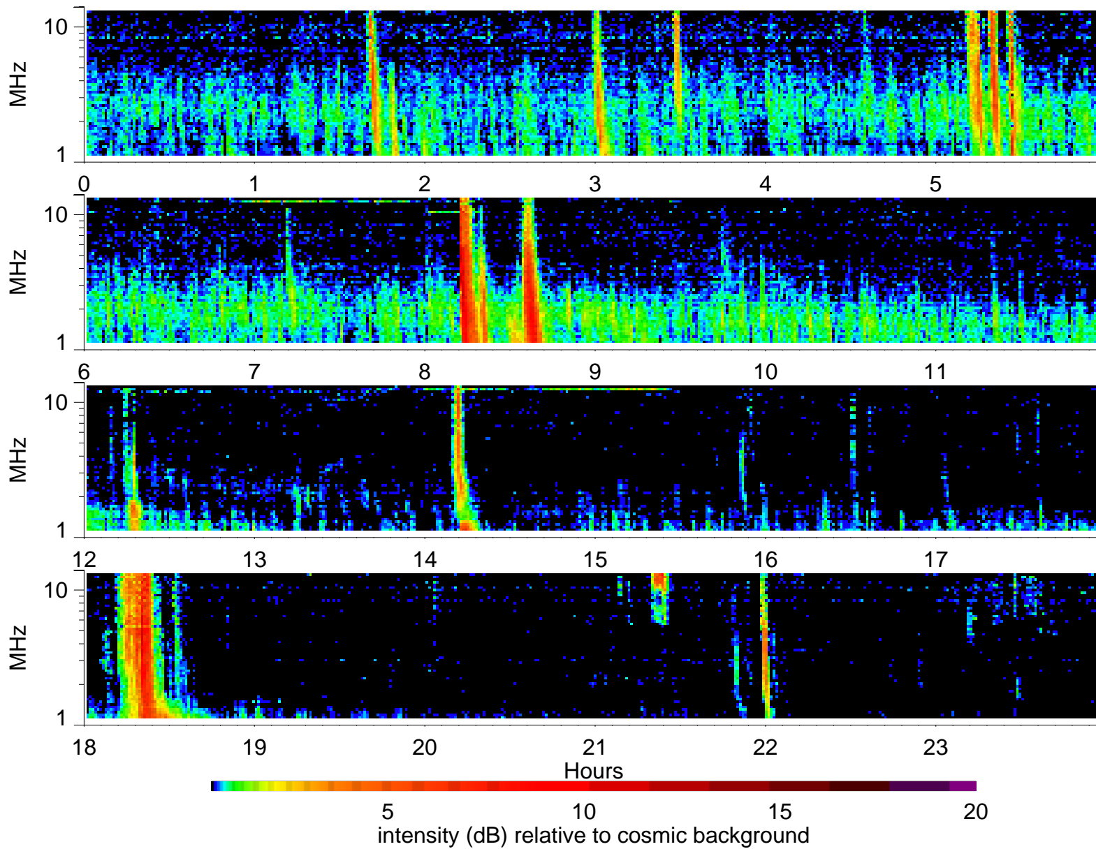
Wind Waves RAD2 receiver: 2001/9/28
