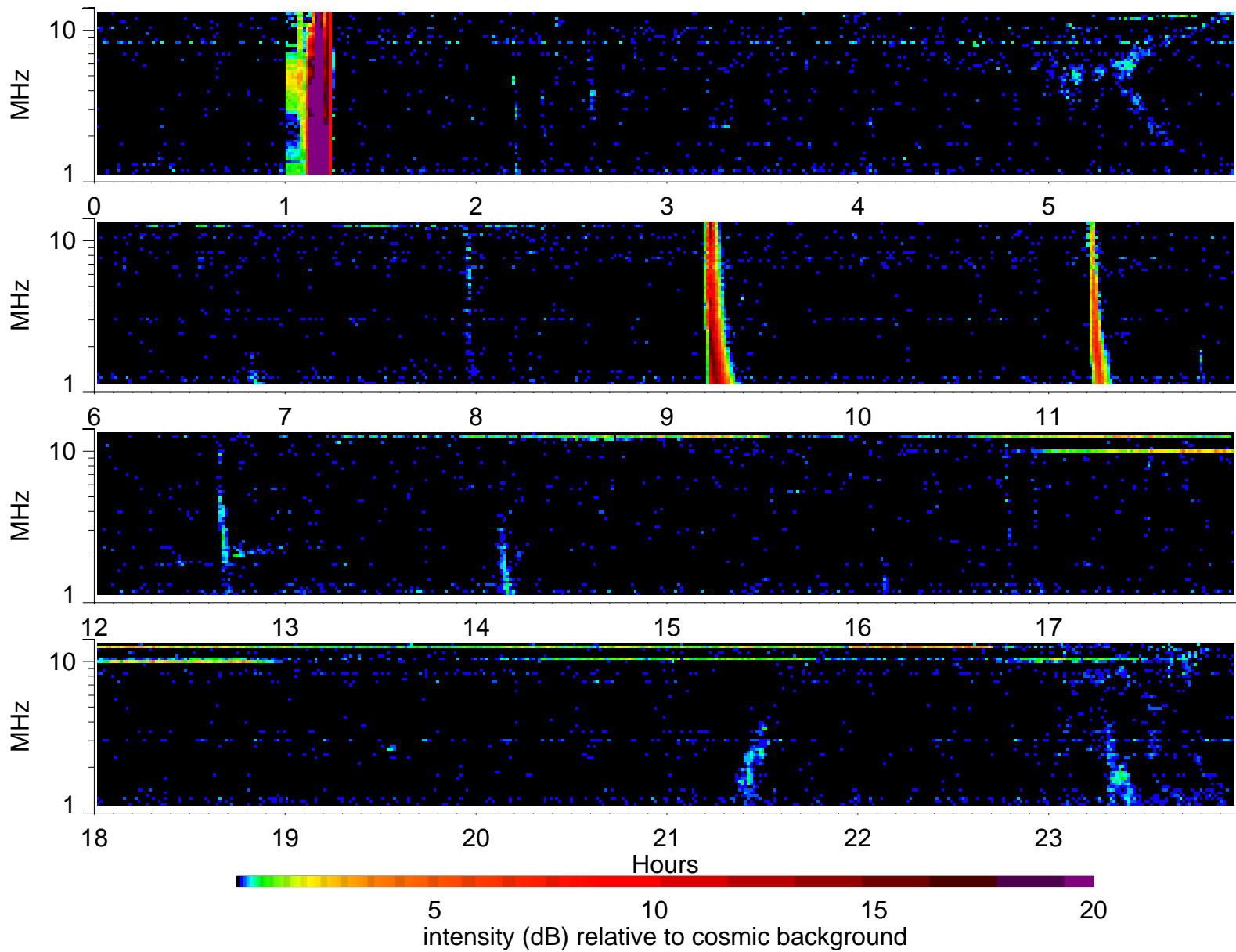
Wind Waves RAD2 receiver: 2001/9/23
