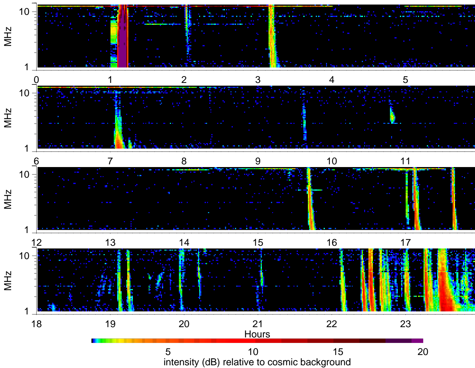
Wind Waves RAD2 receiver: 2001/9/19
