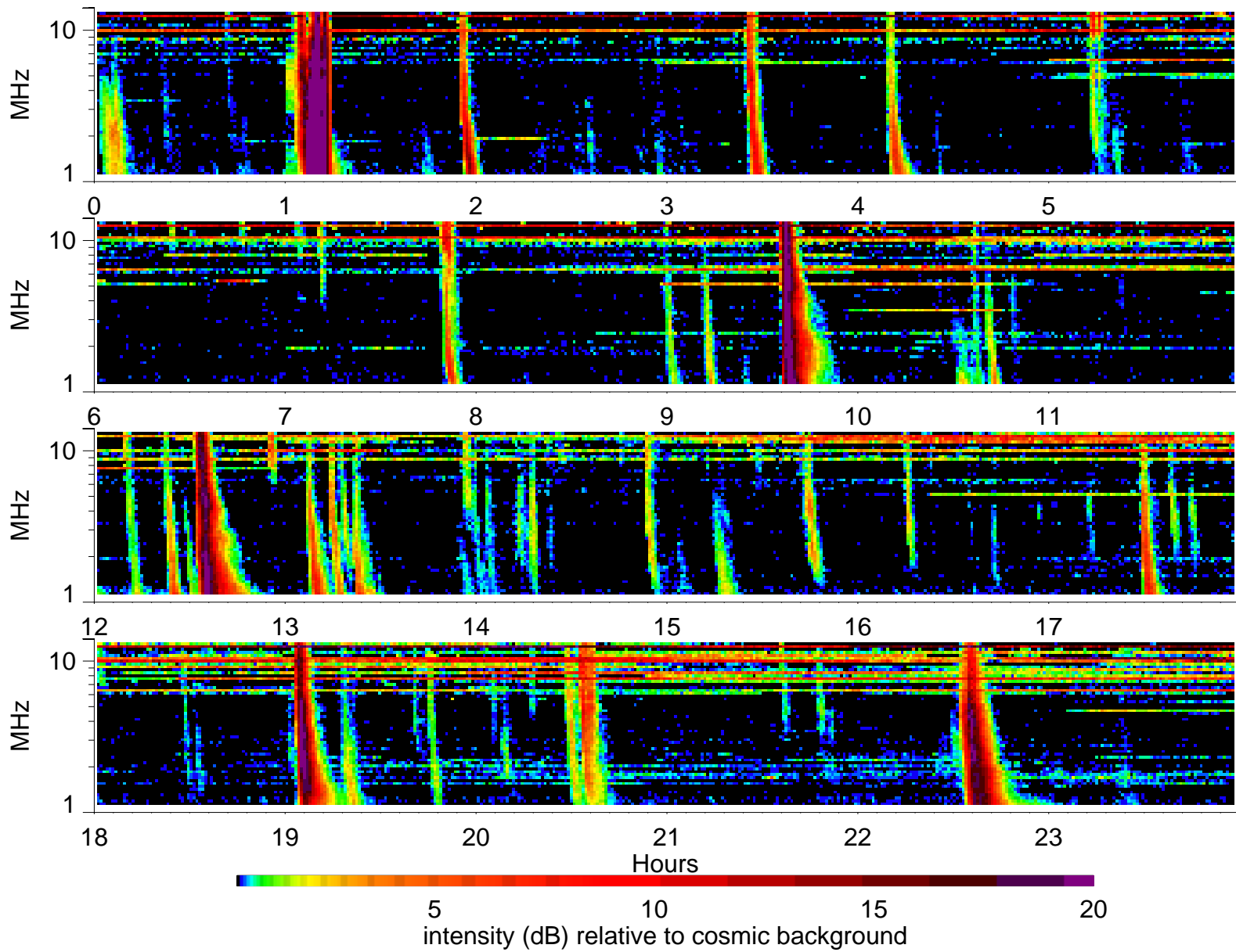
Wind Waves RAD2 receiver: 2001/9/11
