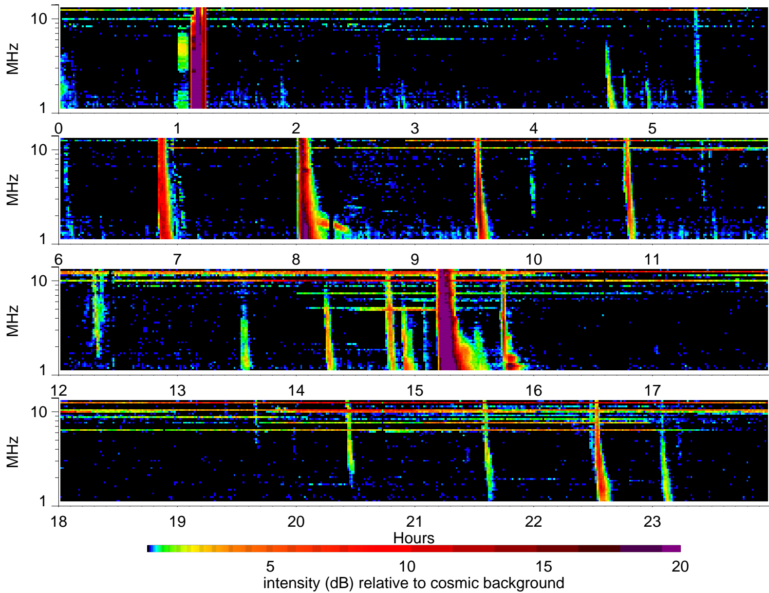
Wind Waves RAD2 receiver: 2001/9/9
