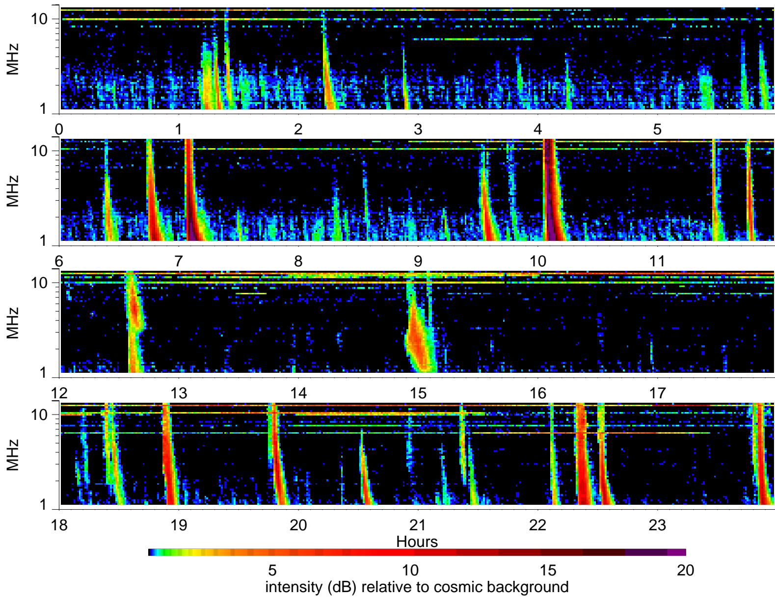
Wind Waves RAD2 receiver: 2001/9/8
