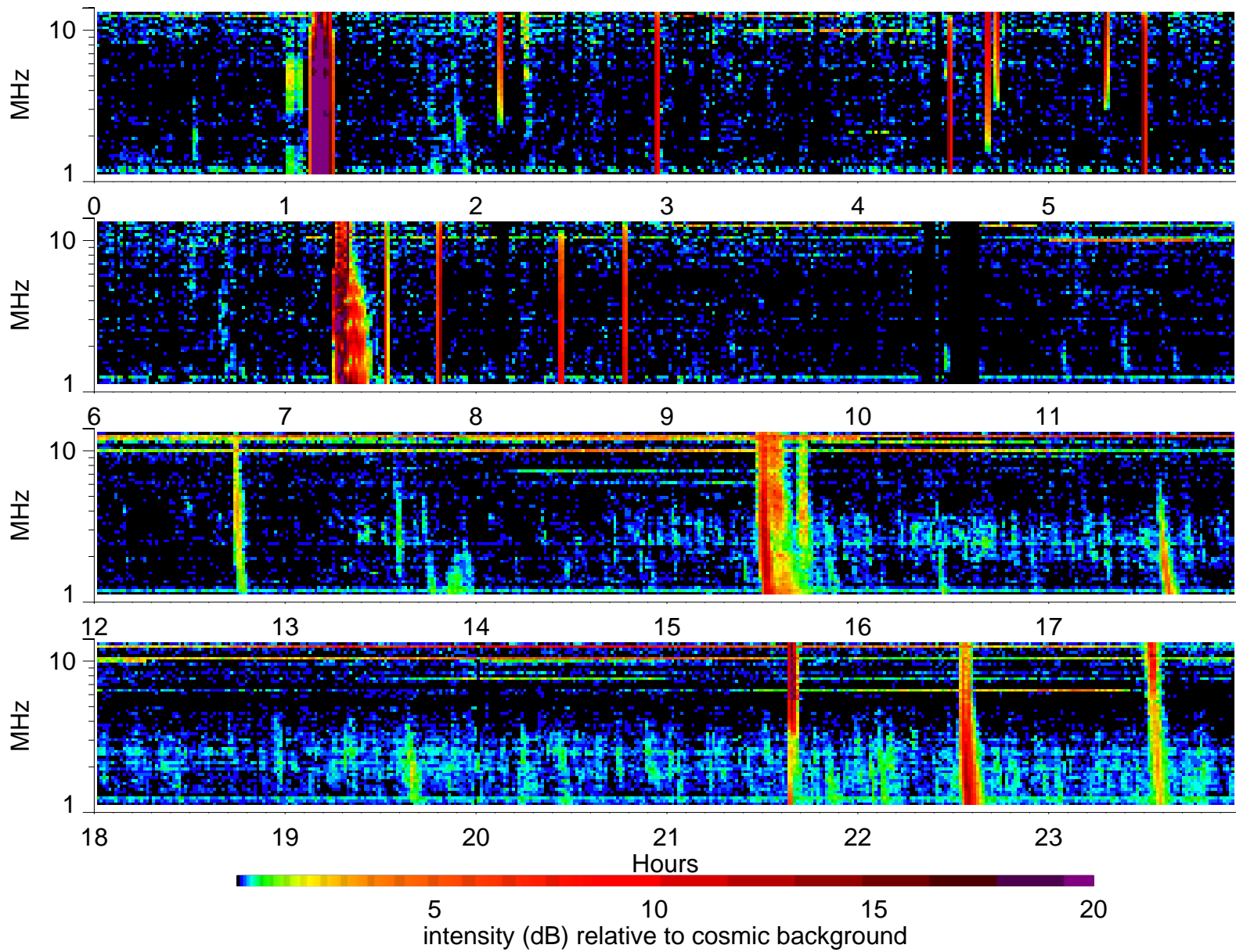
Wind Waves RAD2 receiver: 2001/9/7
