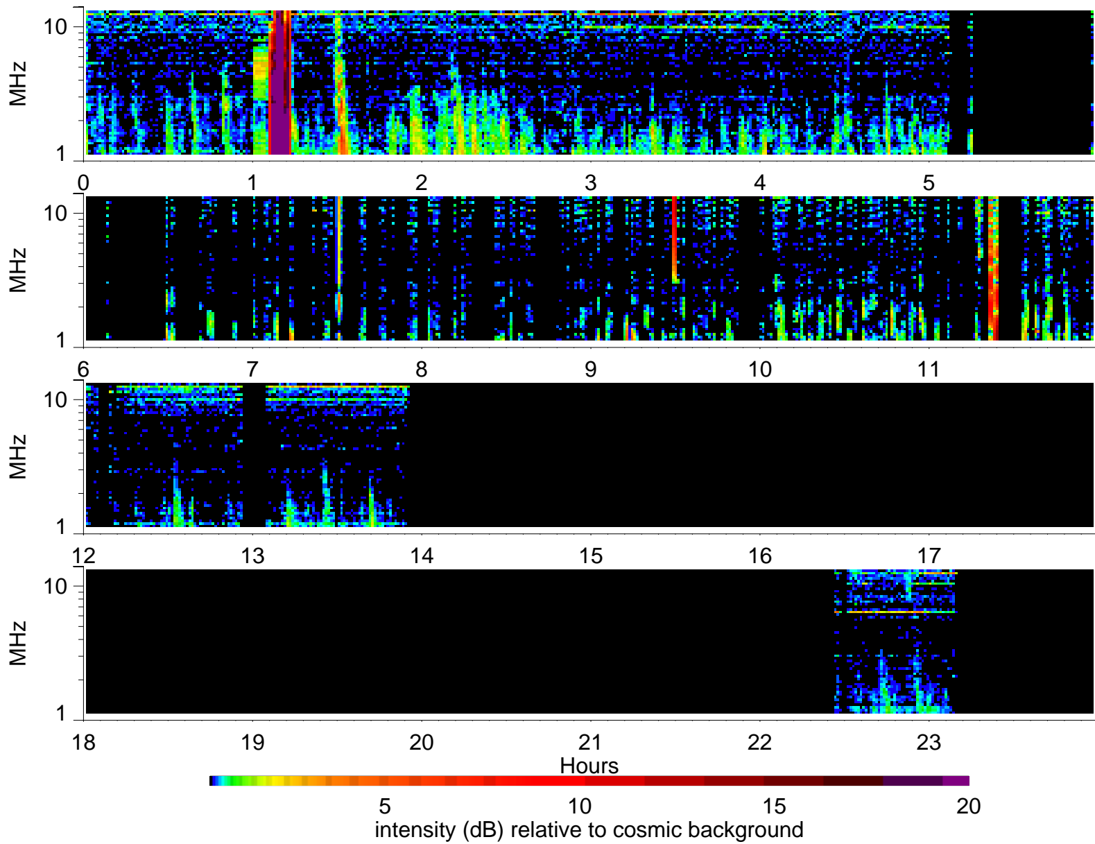
Wind Waves RAD2 receiver: 2001/9/5
