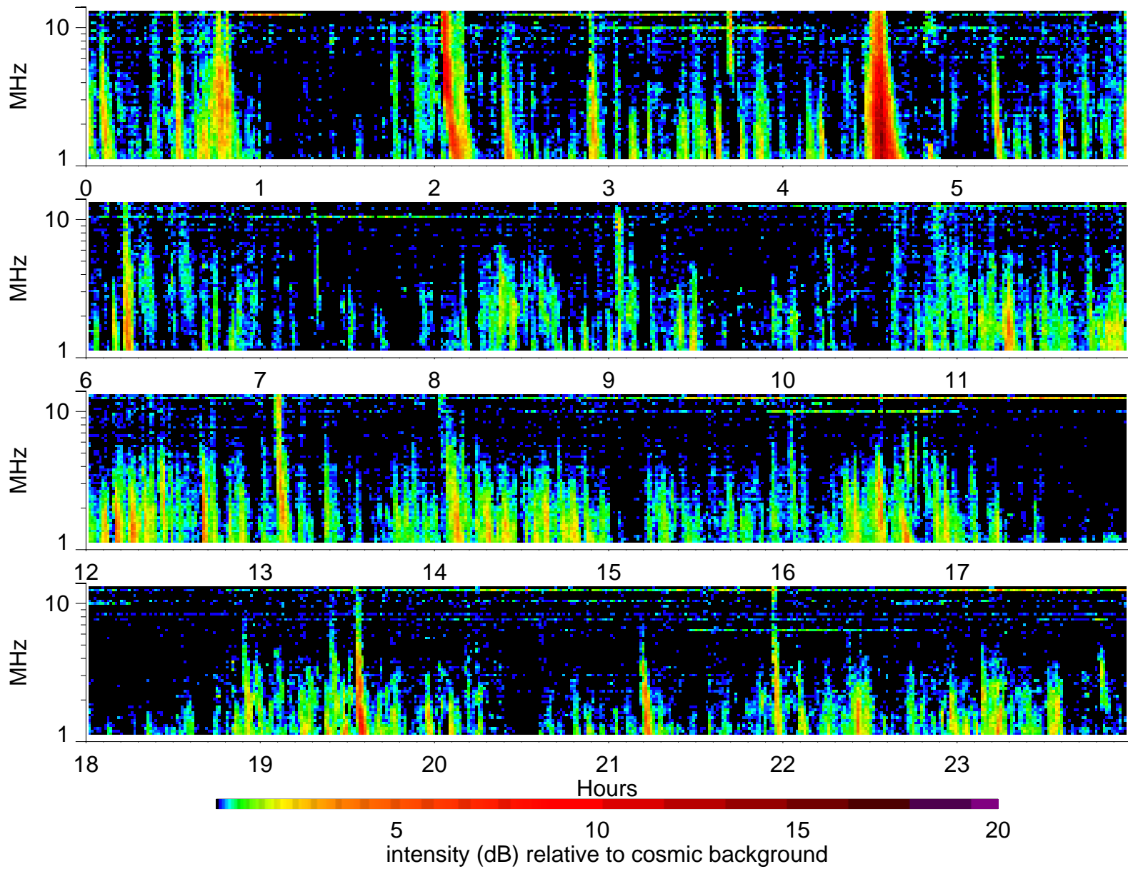
Wind Waves RAD2 receiver: 2001/9/4
