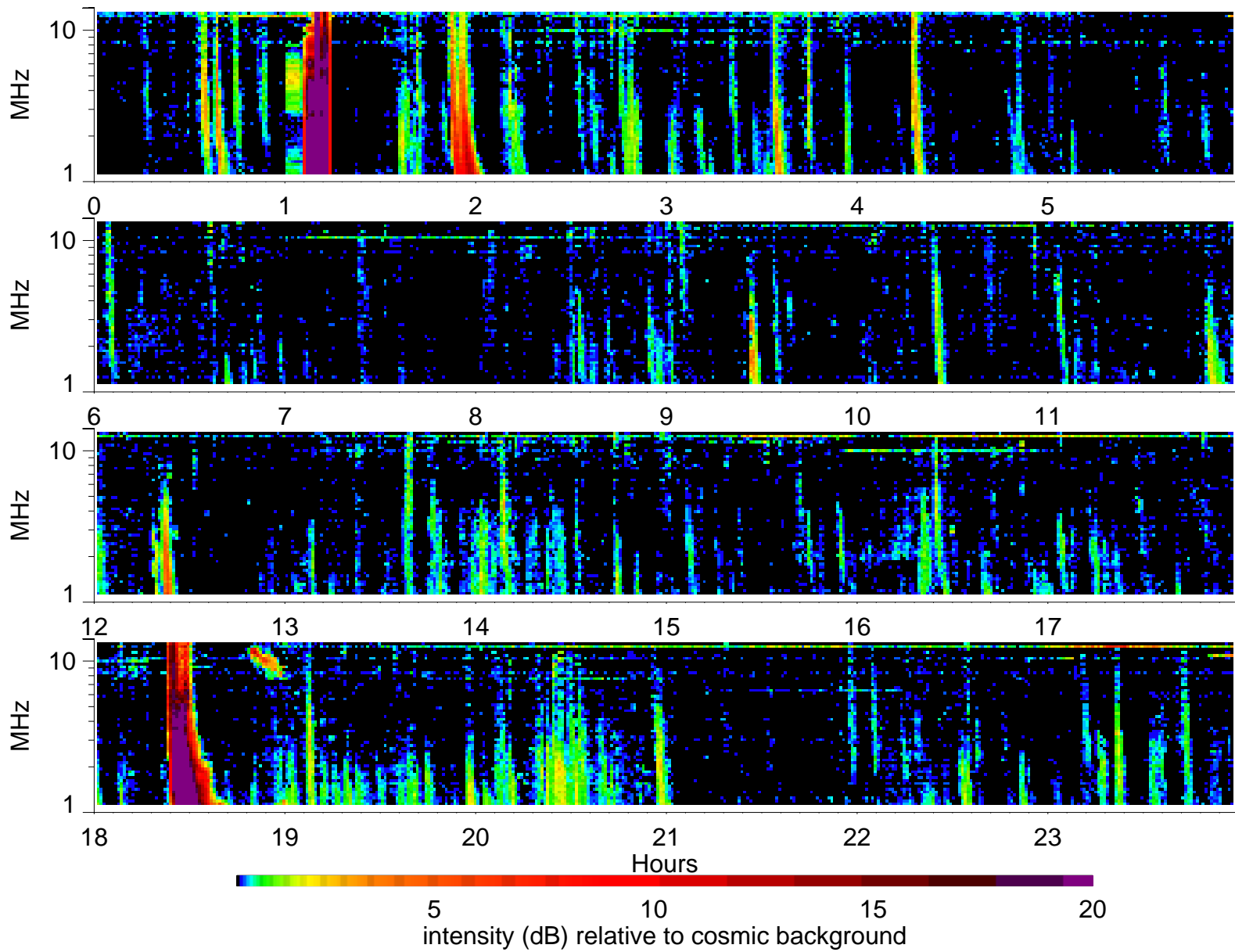
Wind Waves RAD2 receiver: 2001/9/3
